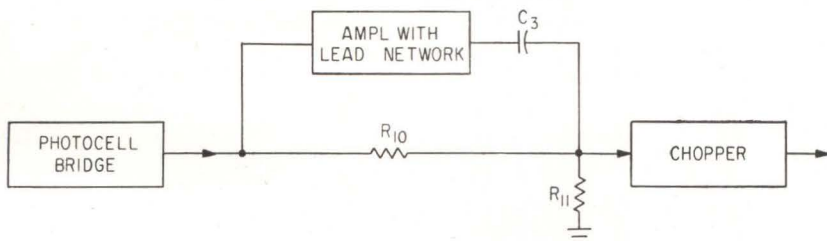
COMPENSATION circuit for dew point servo combines a-c and d-c signals—Fig. 4
