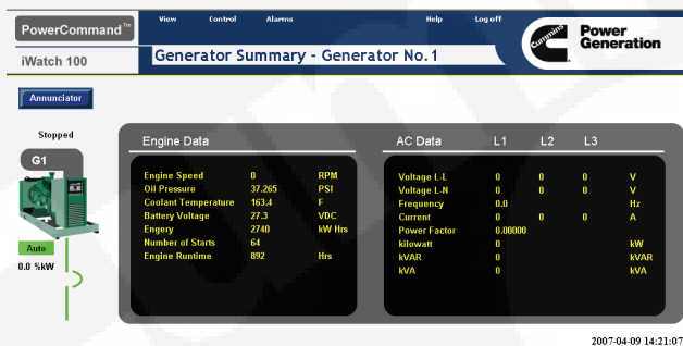
FIGURE 5-4. GENSET AC AND ENGINE DATA PAGE
