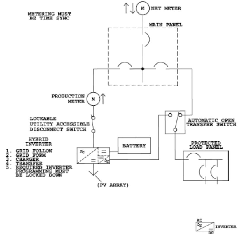
HYBRID EXAMPLE #3b TRANSFER OPTION -BATTERY MAY EXPORT
