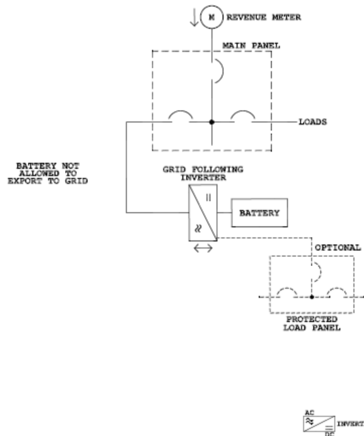
#1b PARALLEL BATTERY
