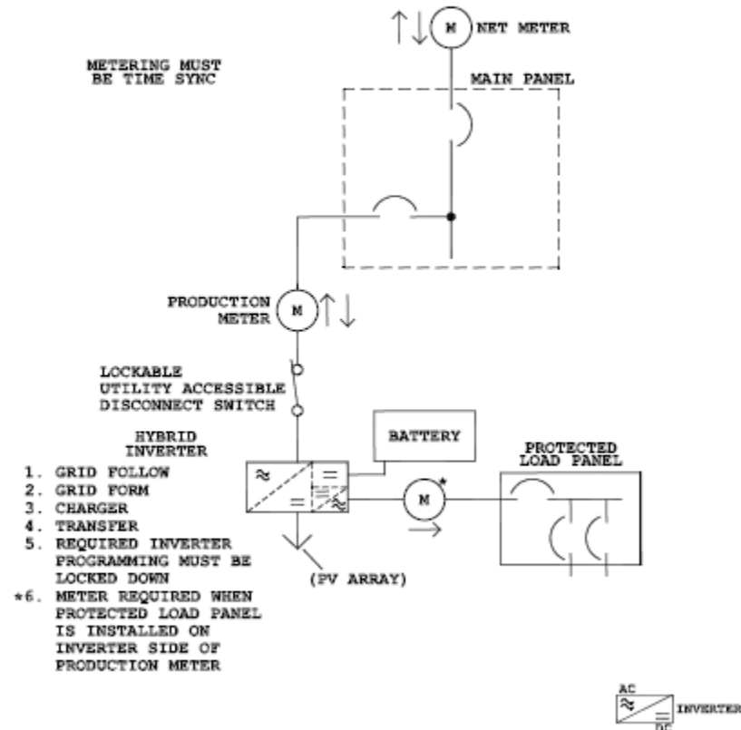
HYBRID EXAMPLE #3a METER OPTION -BATTERY MAY EXPORT
