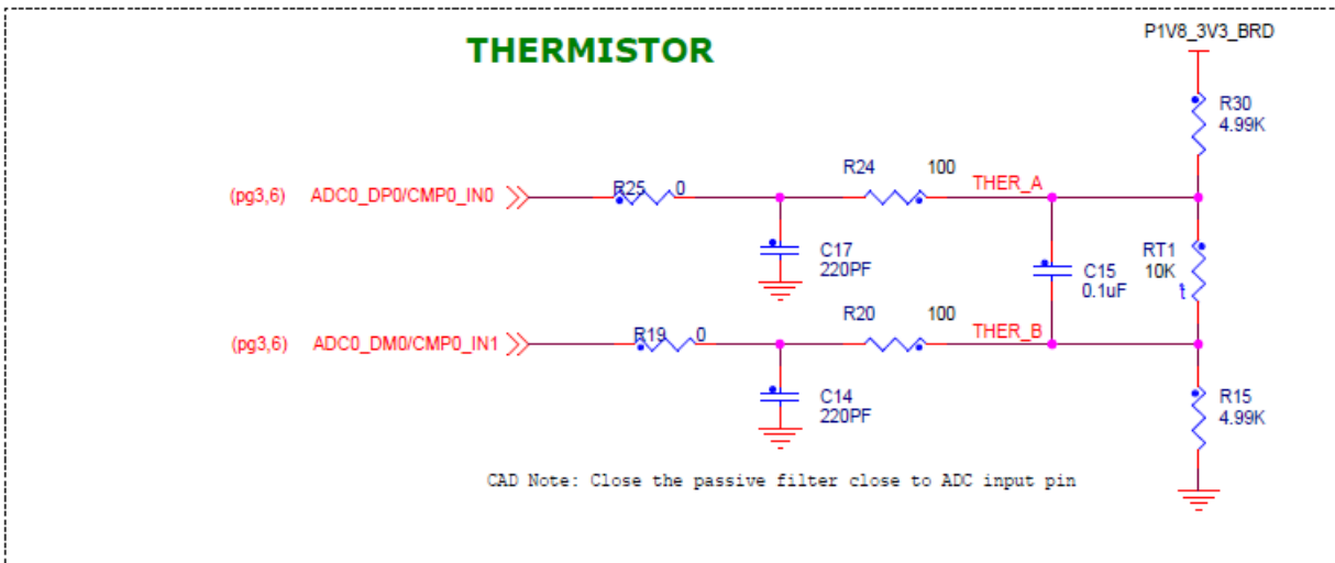
Figure 15. Thermistor circuit
