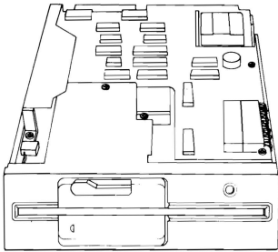
High Capacity Diskette Drive Figure 6 Page 7-14
