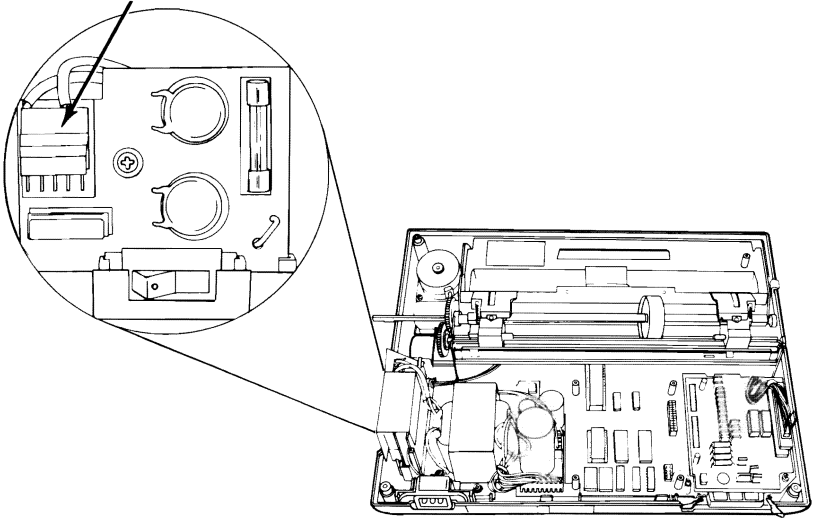
Primary Power Connector
