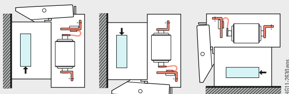
Wall mounting Vertical arrangement
