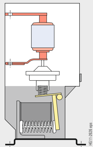
3TL8 vacuum contactor
