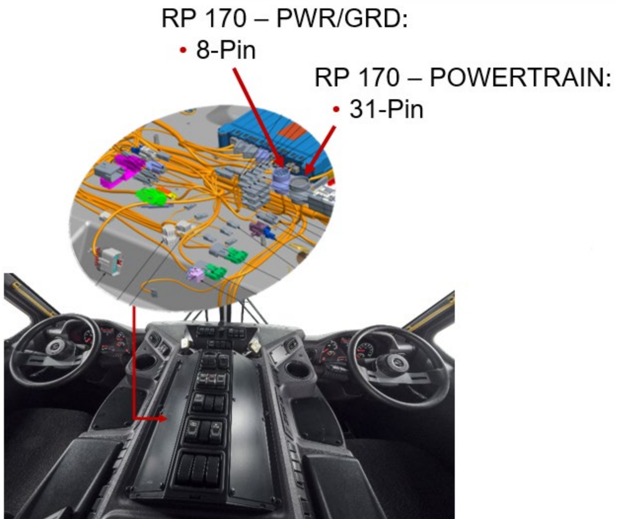
RP170 8-Pin & 31-Pin Connectors
