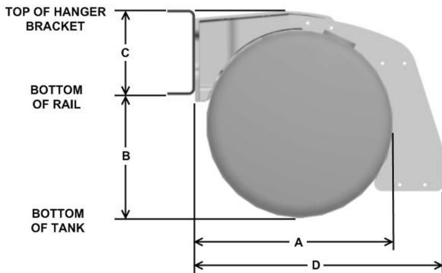
FIGURE 3-31. Fuel Tanks
