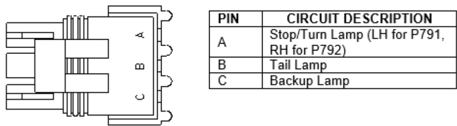
Mating Connector: Packard PN 12015713
