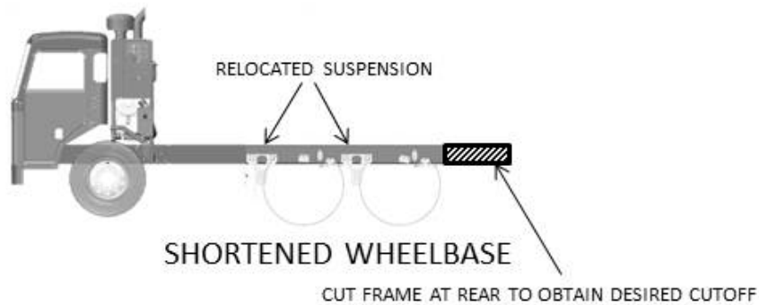
FIGURE 5-1. Wheelbase Customization
