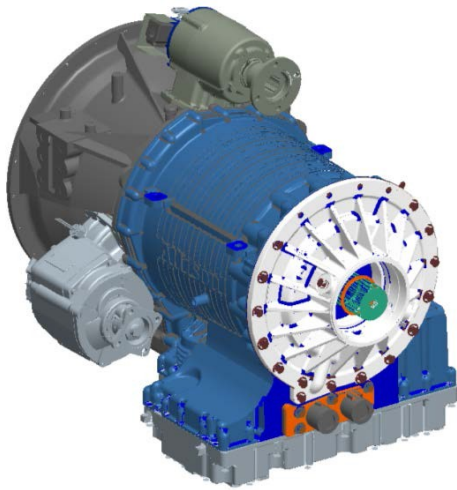
FIGURE 7-3. Allison 4000 Series
