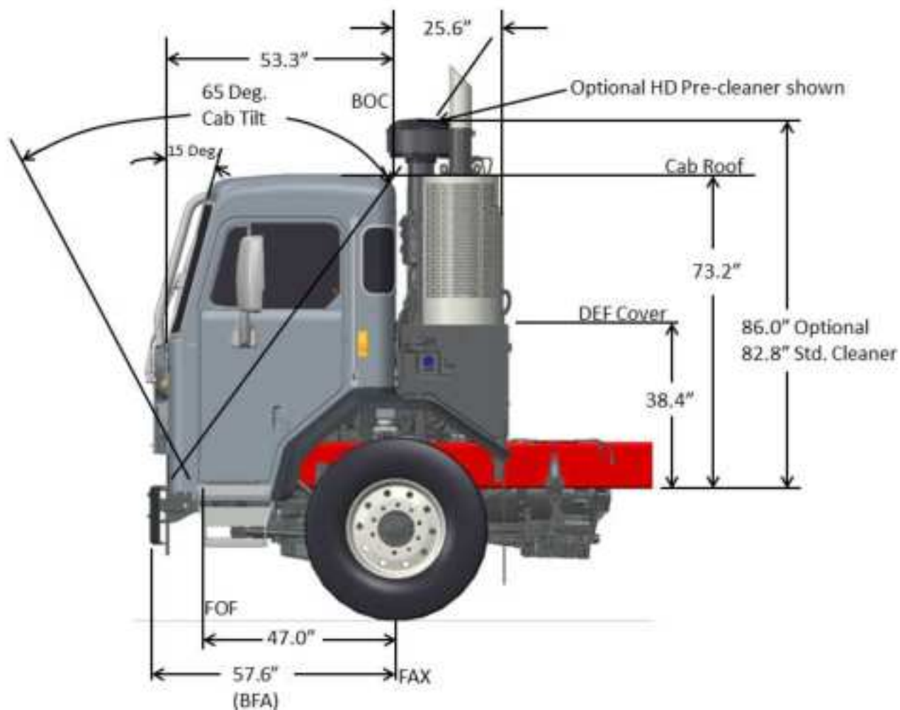
FIGURE 3-2. 520 Cab Dimensions
