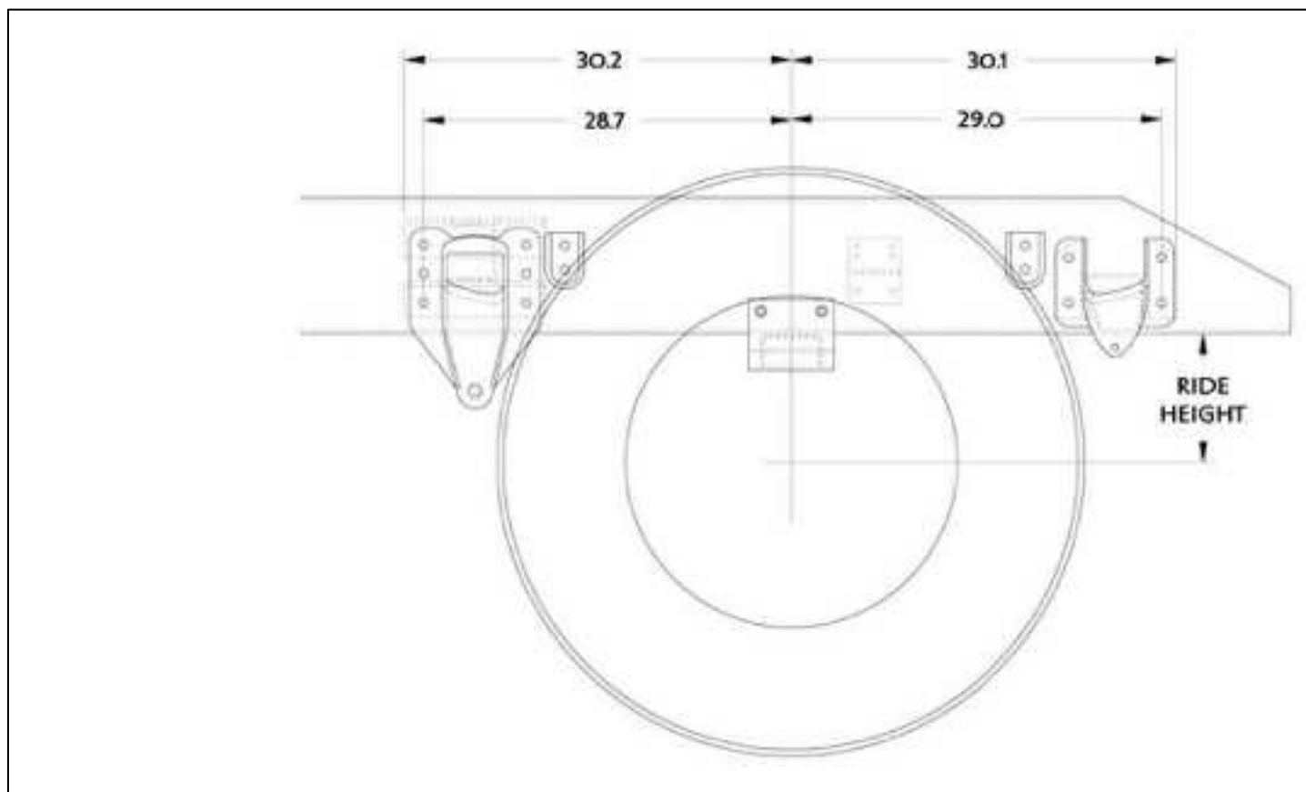
FIGURE 3-5. Reyco 79KB Frame Drilling (Dimensions In Inches)
