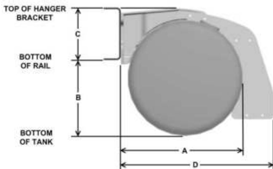
FIGURE 3-31. Fuel Tanks
