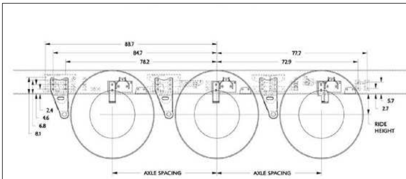
FIGURE 3-8. Neway ADZ 369/378 Frame Drilling (Dimensions In Inches)
