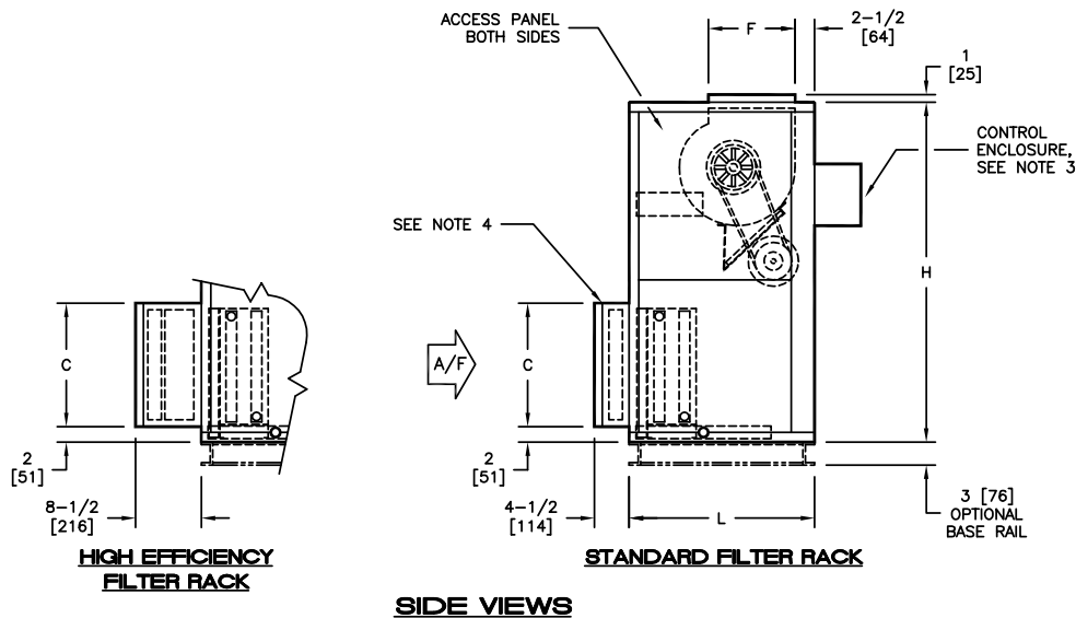
SIDE VIEWS
