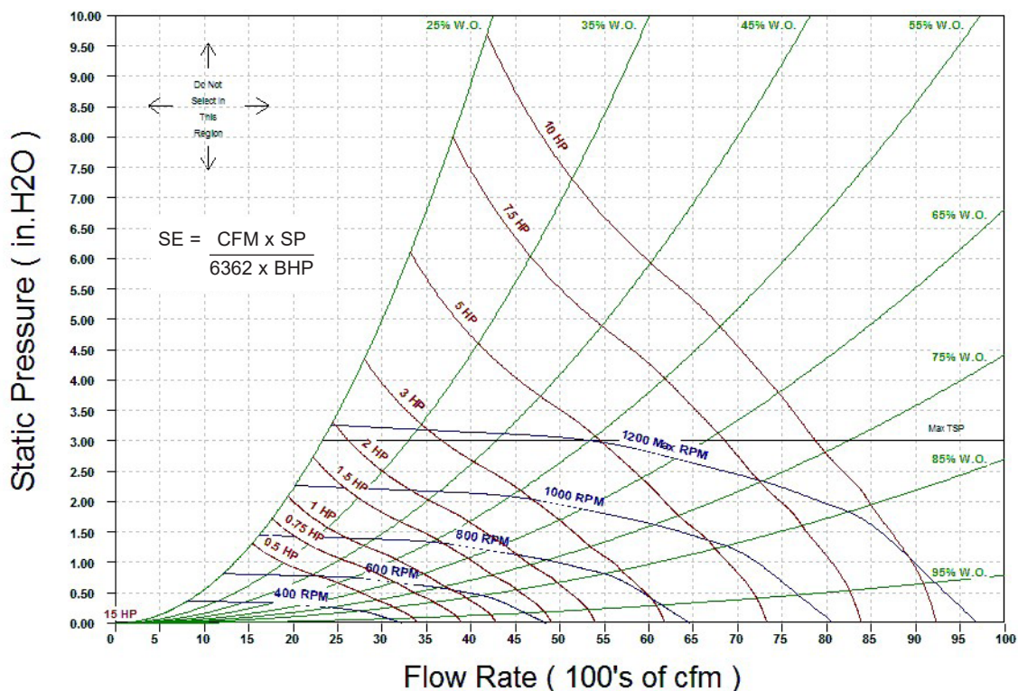
UNIT SIZE 40 (FAN 1511R)
