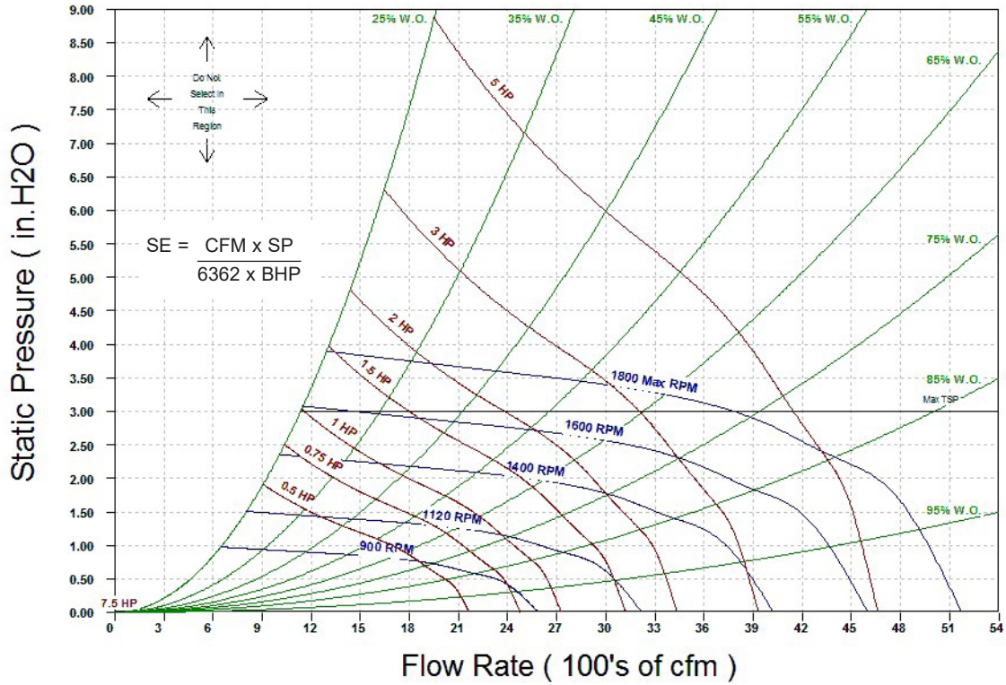
UNIT SIZE 16 (FAN 1008R)
