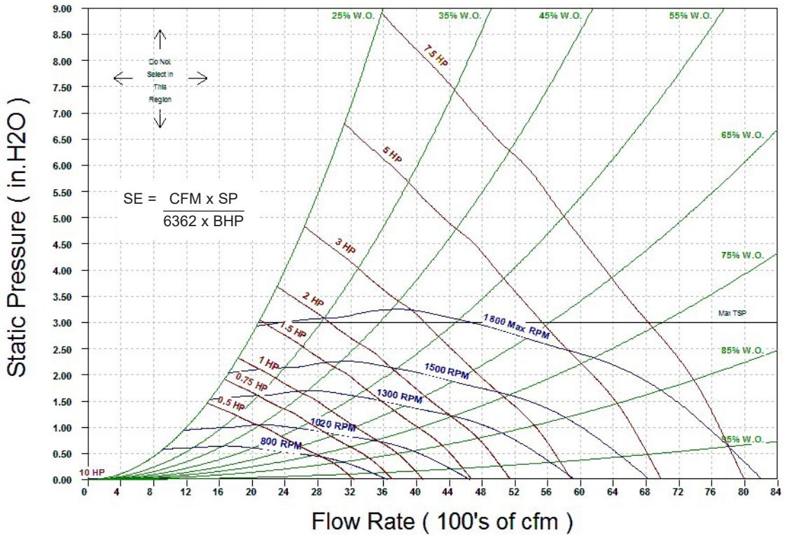
UNIT SIZE 20 (FAN 1010R)
