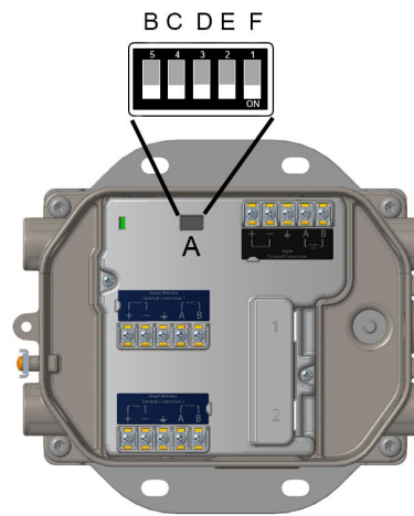
Figure 2-3: DIP Switch Identification
