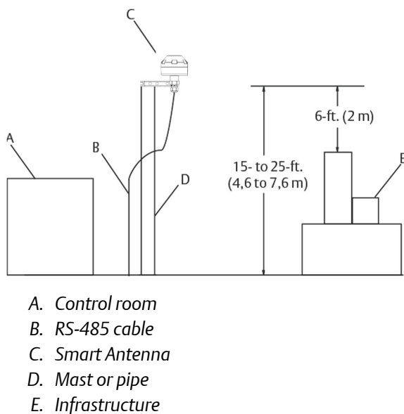
Figure 3-3: Mounting Location
