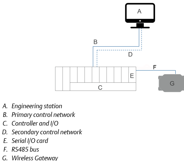
Figure 5-2: RS485 Architecture
