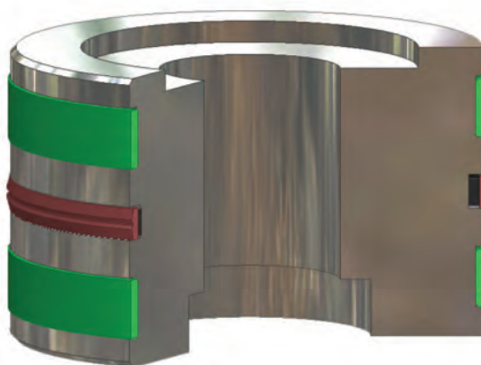
BP installed in Piston Gland
