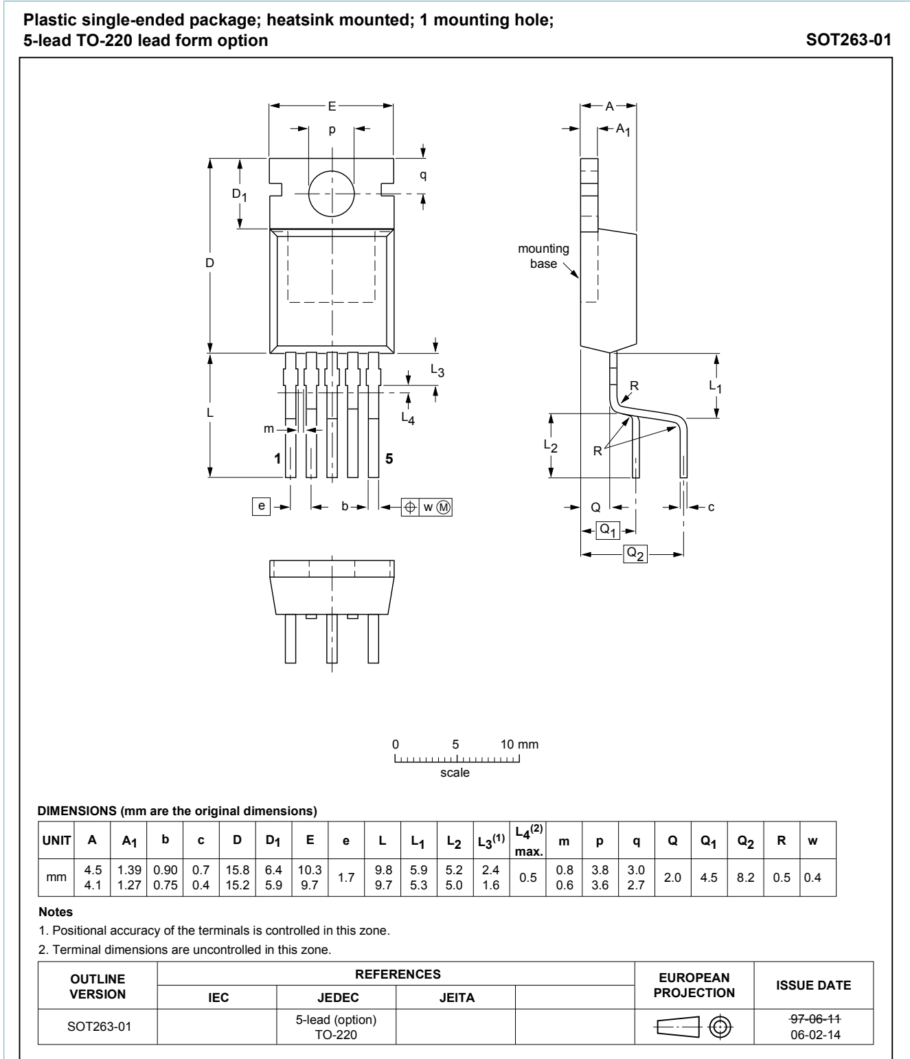
Fig. 1. Package outline TO-220-5 option (SOT263-01)
