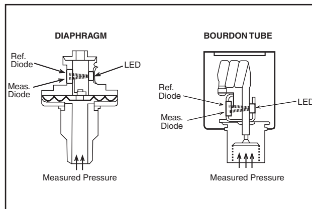
Figure 1. Sensor Cutaway
