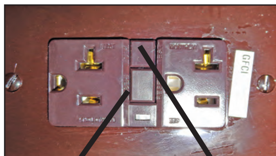
Figure 9-3: GFCI receptacle
