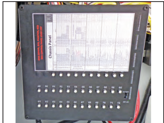
Figure 9-6: Circuit breakers
