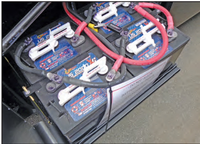
Figure 9-9: House batteries
