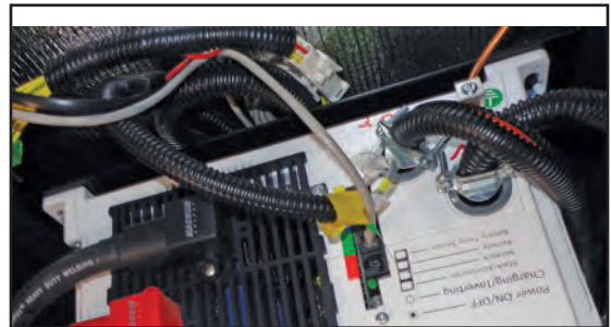
Figure 9-4: Converter/Inverter
