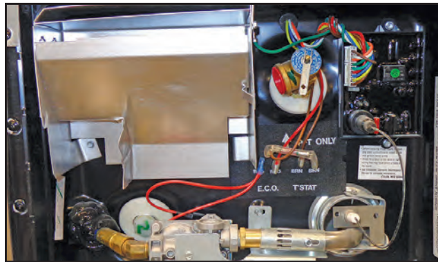
Figure 5-8: Water heater
