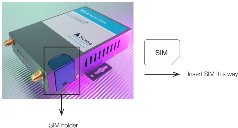
Figure 9. SIM holder
