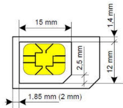
Figure109. SIM card dimensions
