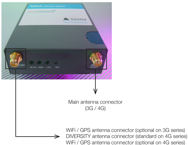
Figure 11. Antenna connectors
