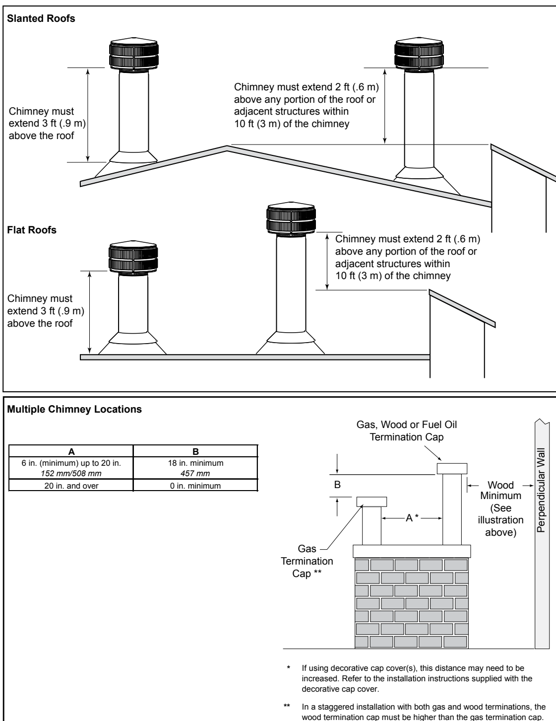
Figure 6.1 Multiple Chimneys
