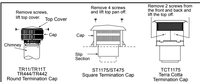
Figure 11.1 Chimney & Termination Cap Cleaning
