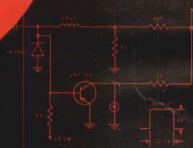
ONE SHOT MULTIVIBRATOR WITH HIGH GAIN INVERTER
