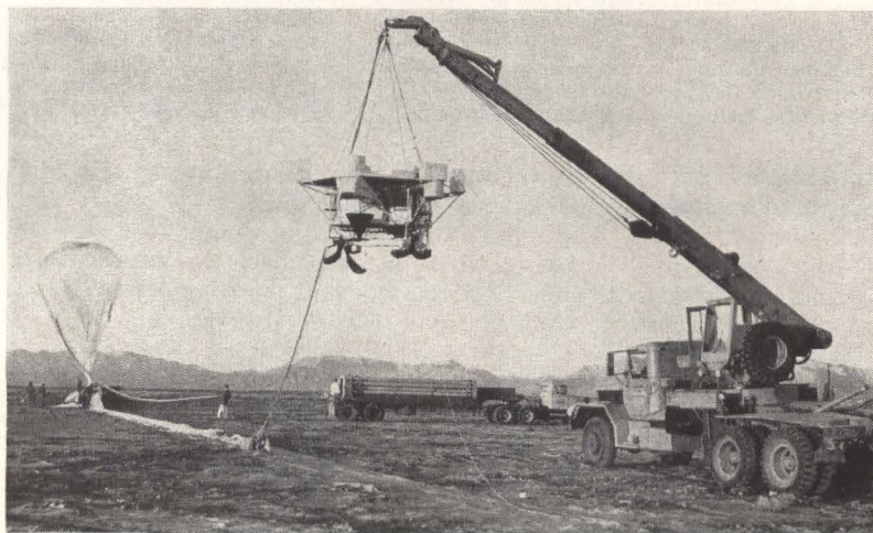
Recent tests in the New Mexico desert measured cosmic ray background for calibration of radioisotope distance measuring devices
