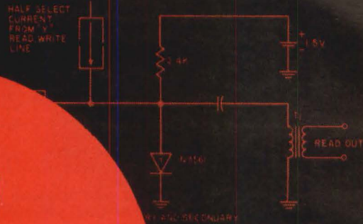
MEMORY CELL
