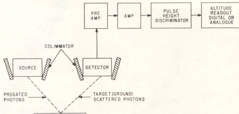
Reflections are sensed by multiplier phototube in scintillator system or by p-n junction in solid-state version
