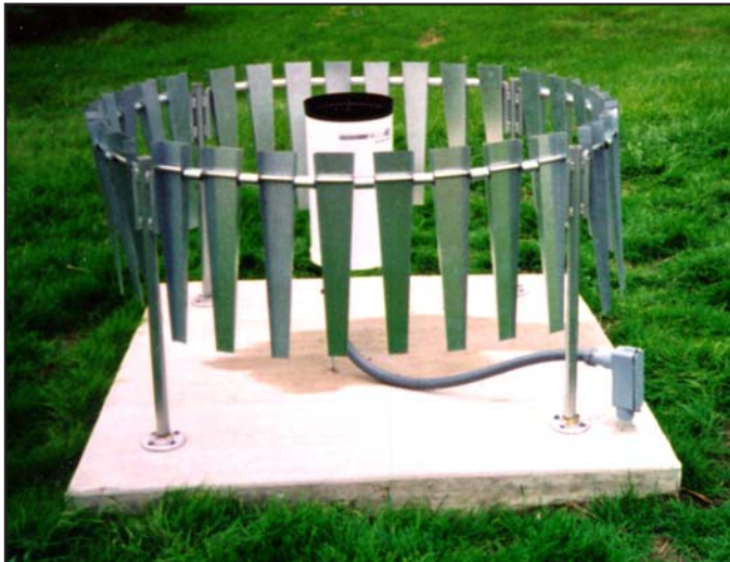
260-952 Precipitation Gauge Wind Screen
