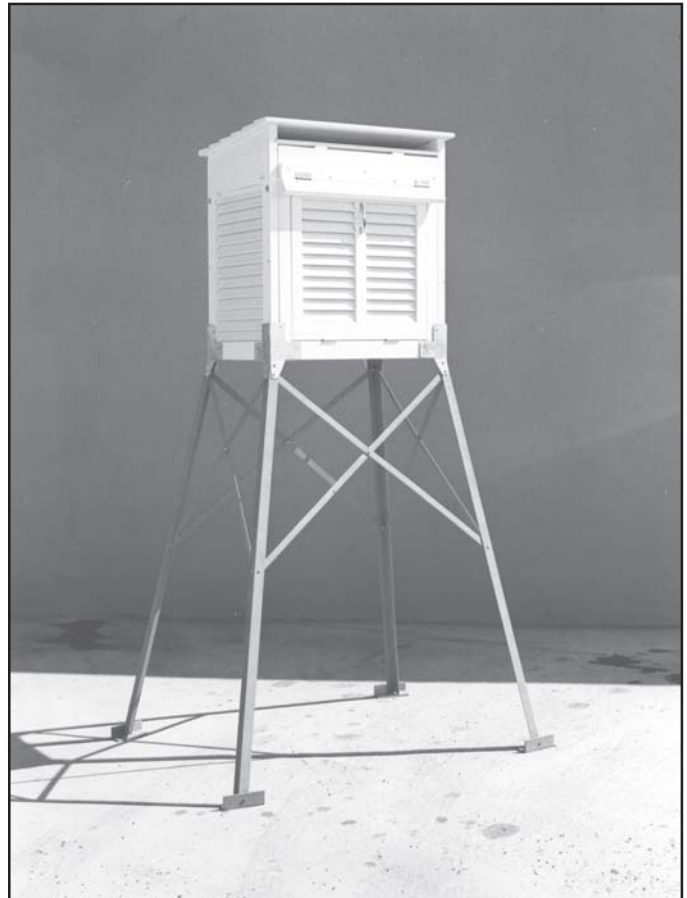
380-605 Large Instrument Shelter with 380-609 Metal Leg Kit
