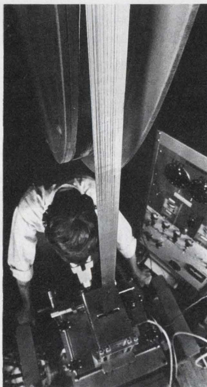
1. Long continuous ribbons of silicon crystal grown at Mobil Tyco Labs may lead to mass-produced low-cost solar cell arrays.
