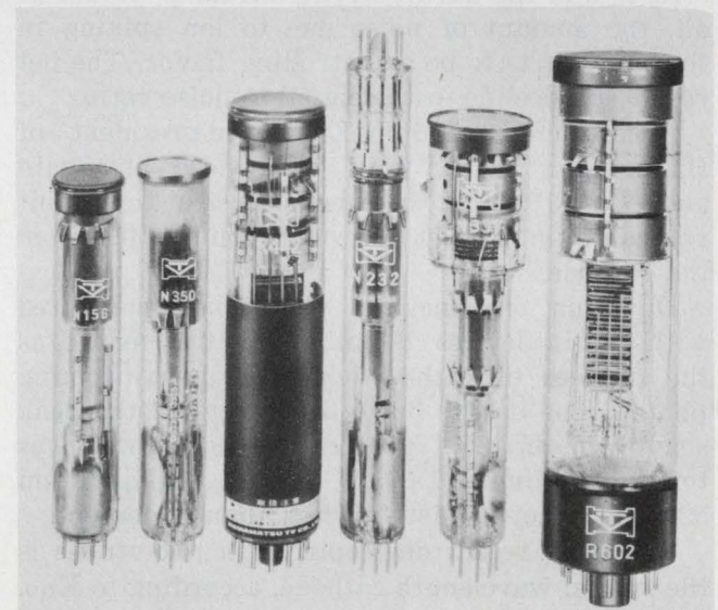
Phototubes from Hamamatsu such as these can produce gains of 100 to 100 million. Used for very low light level detection where good signal-to-noise ratios are important, their best sensitivity is at about 400 nm.
