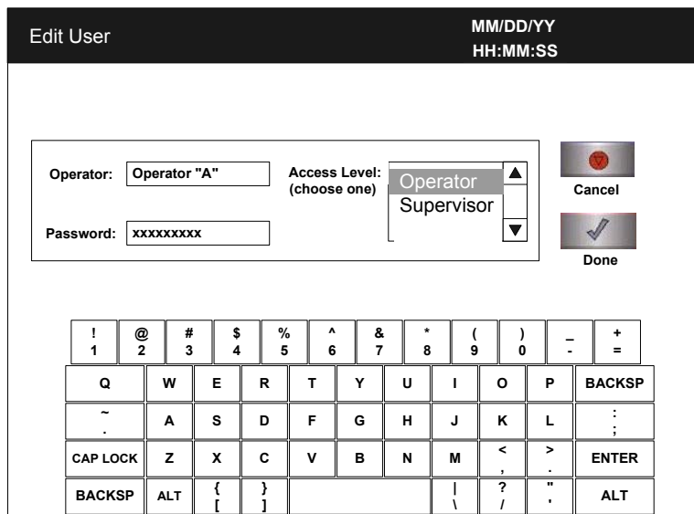
Figure 31. Edit User
