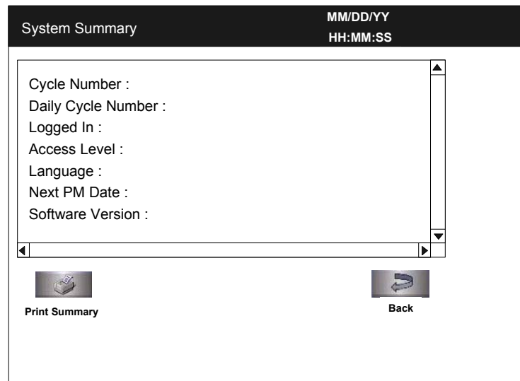
Figure 33. System Summary
