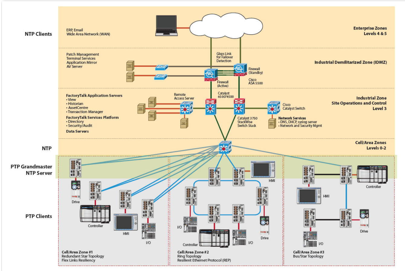
Figure 6 - Example Architecture
