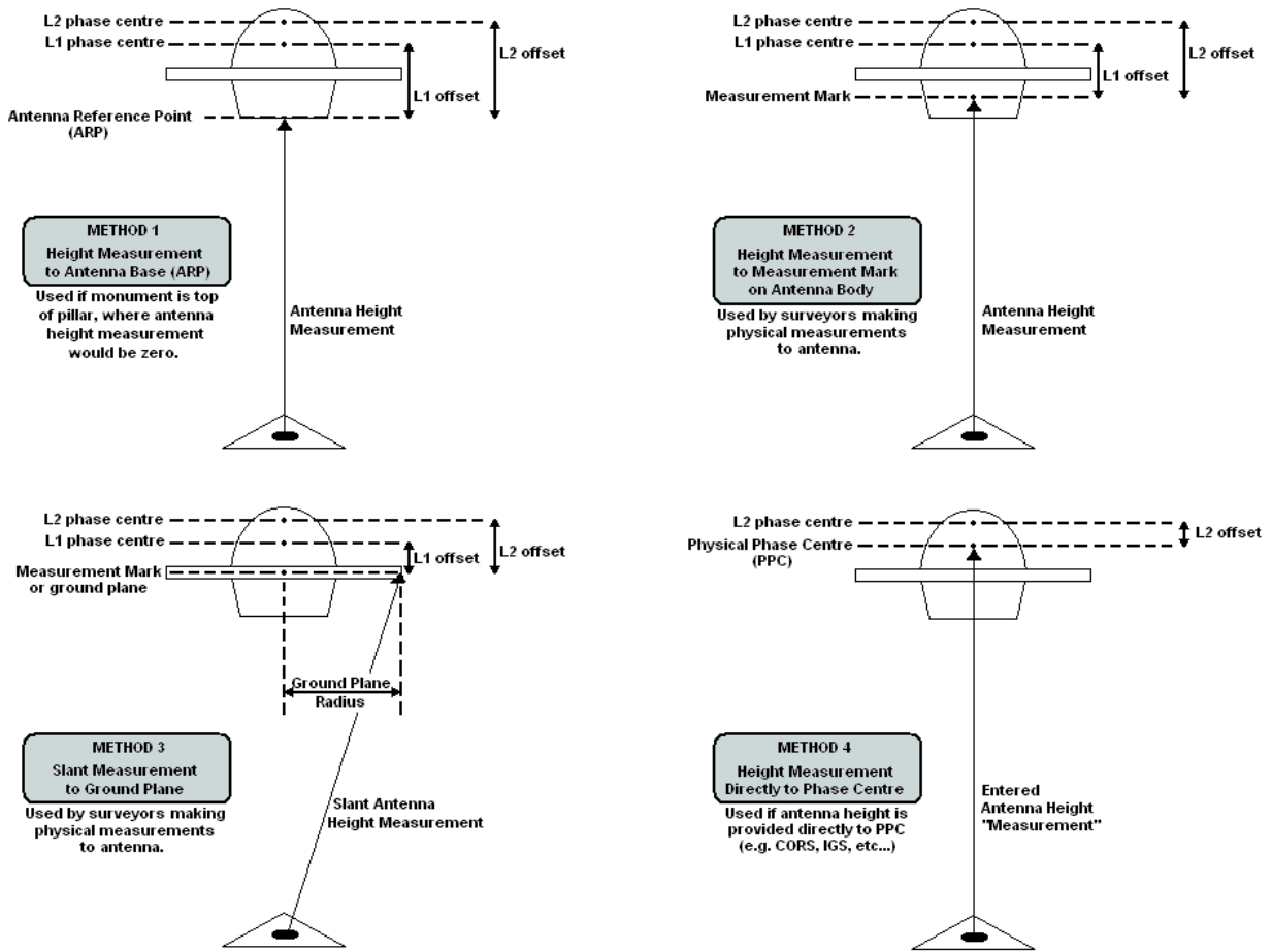
Figure 7: Antenna Measurements
