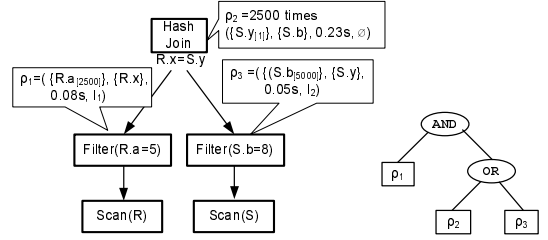
Figure 1. Execution plan and AND/OR request tree.
