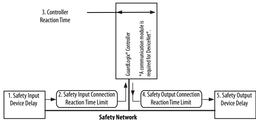
Figure 24 - Logix System Worst-case Reaction Time for Simple Input to Logic to Output
