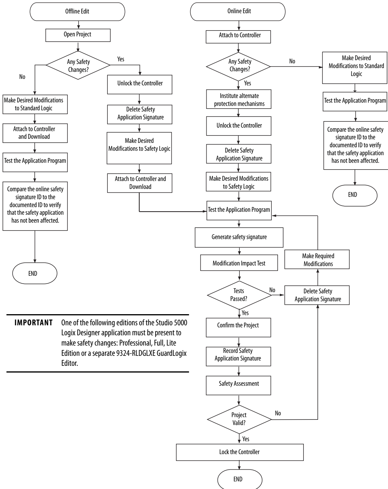
Figure 17 - Online and Offline Edit Process
