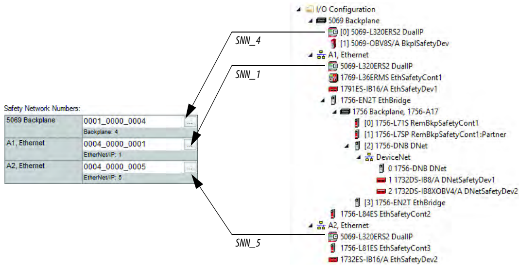
Figure 10 - Controller Organizer
