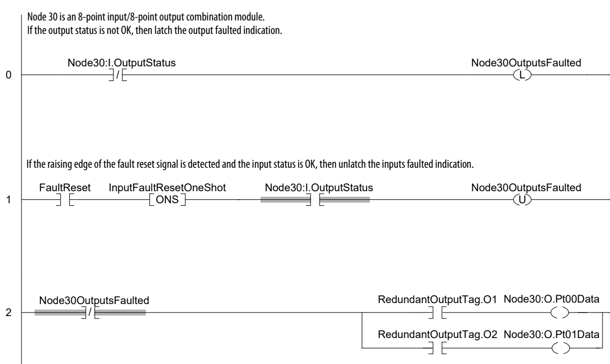
Figure 30 - Ladder Diagram Example 3
