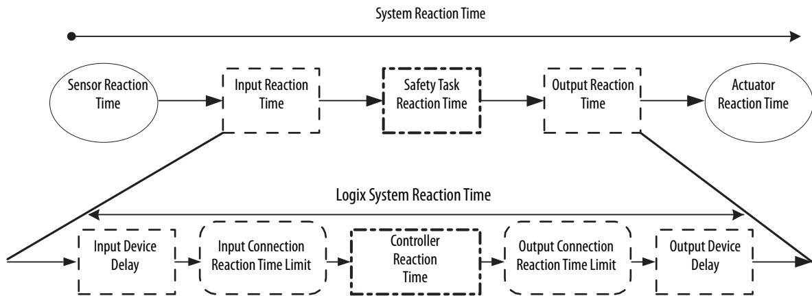
Figure 23 - System Reaction Time
