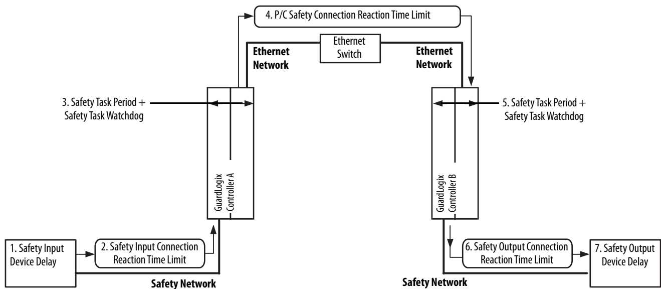
Figure 25 - Logix System Reaction Time for Input to Controller A Logic to Controller B Logic to Output Chain
