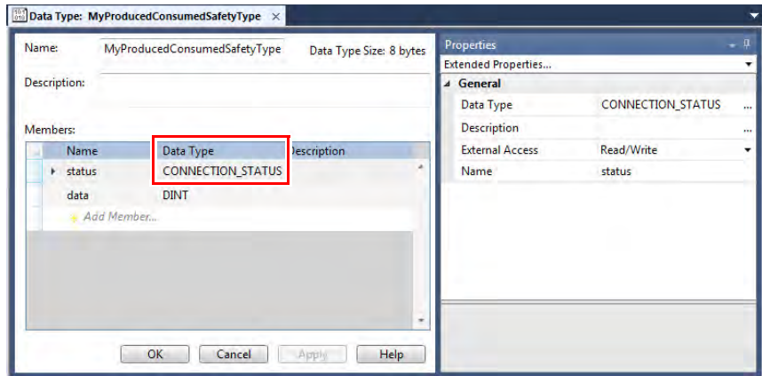
Figure 18 - Data Type Dialog Box
