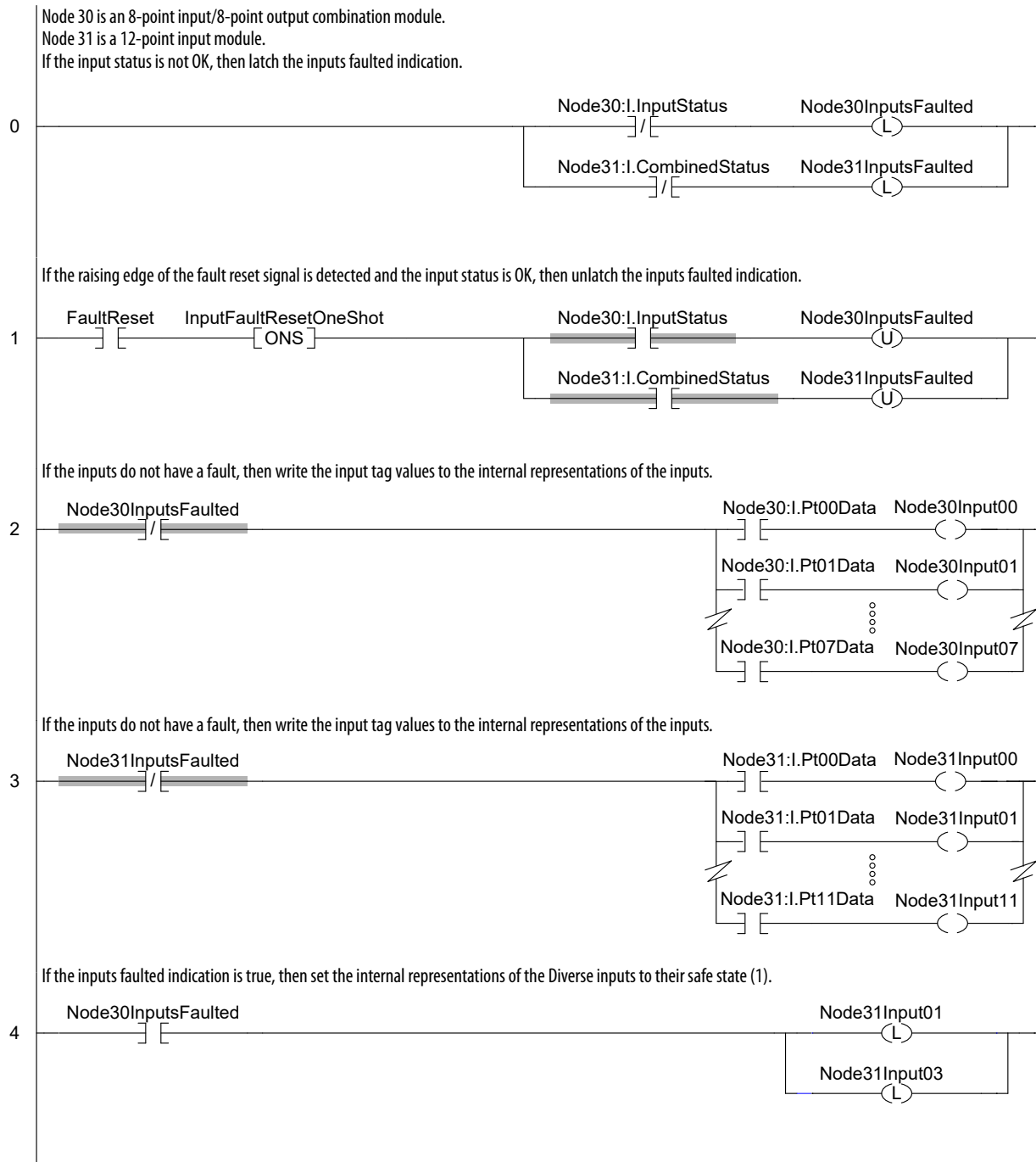
Figure 28 - Ladder Diagram Example 2
