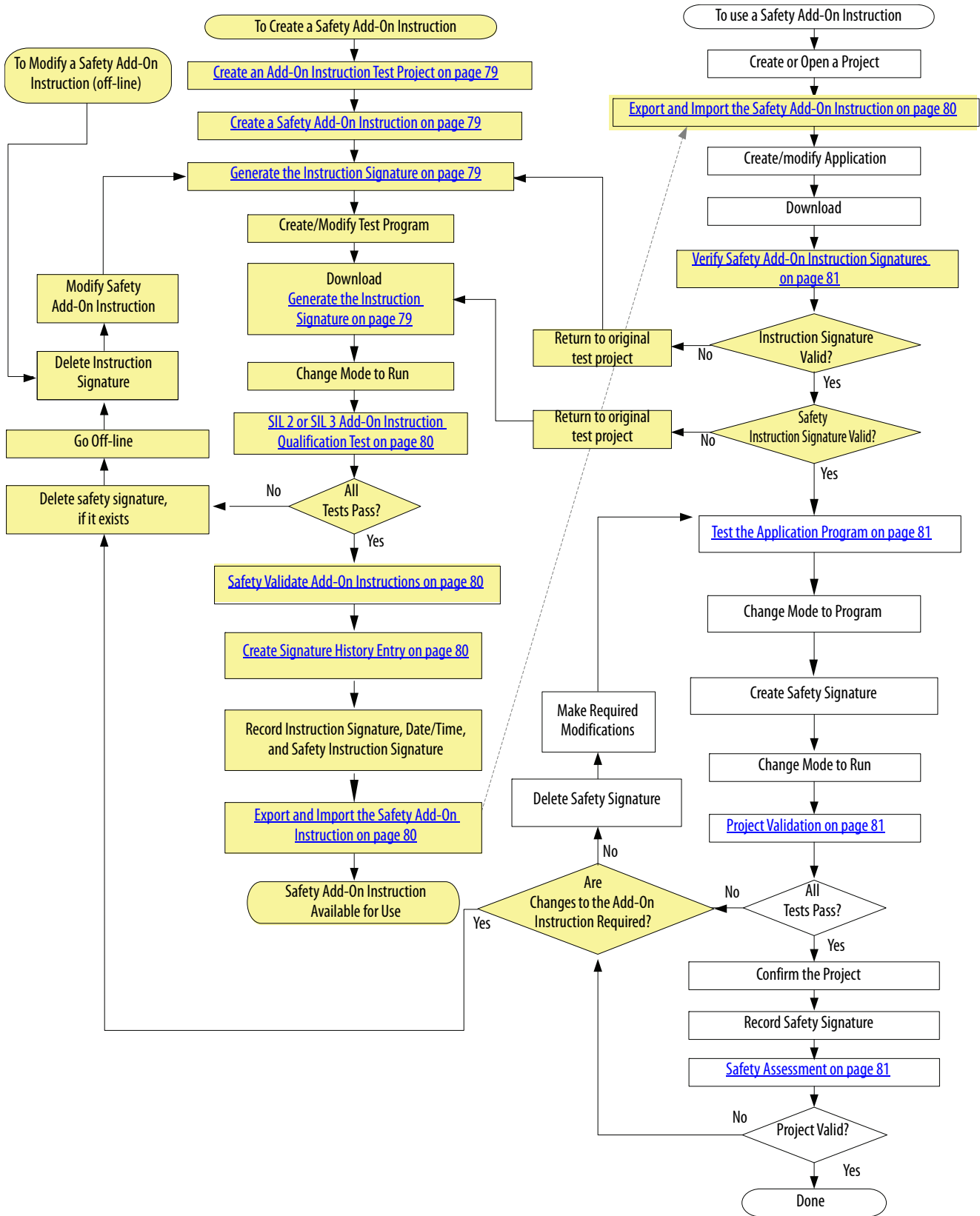
Figure 19 - Flowchart for Creating and Using Safety Add-On Instructions
