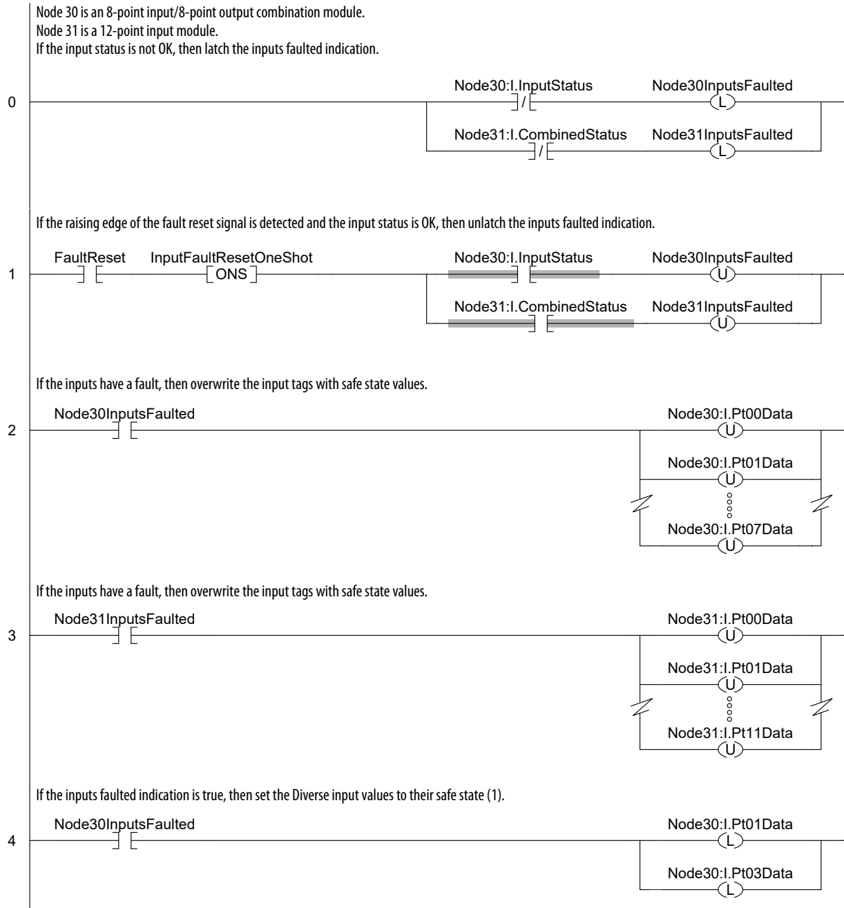
Figure 27 - Ladder Diagram Example 1
