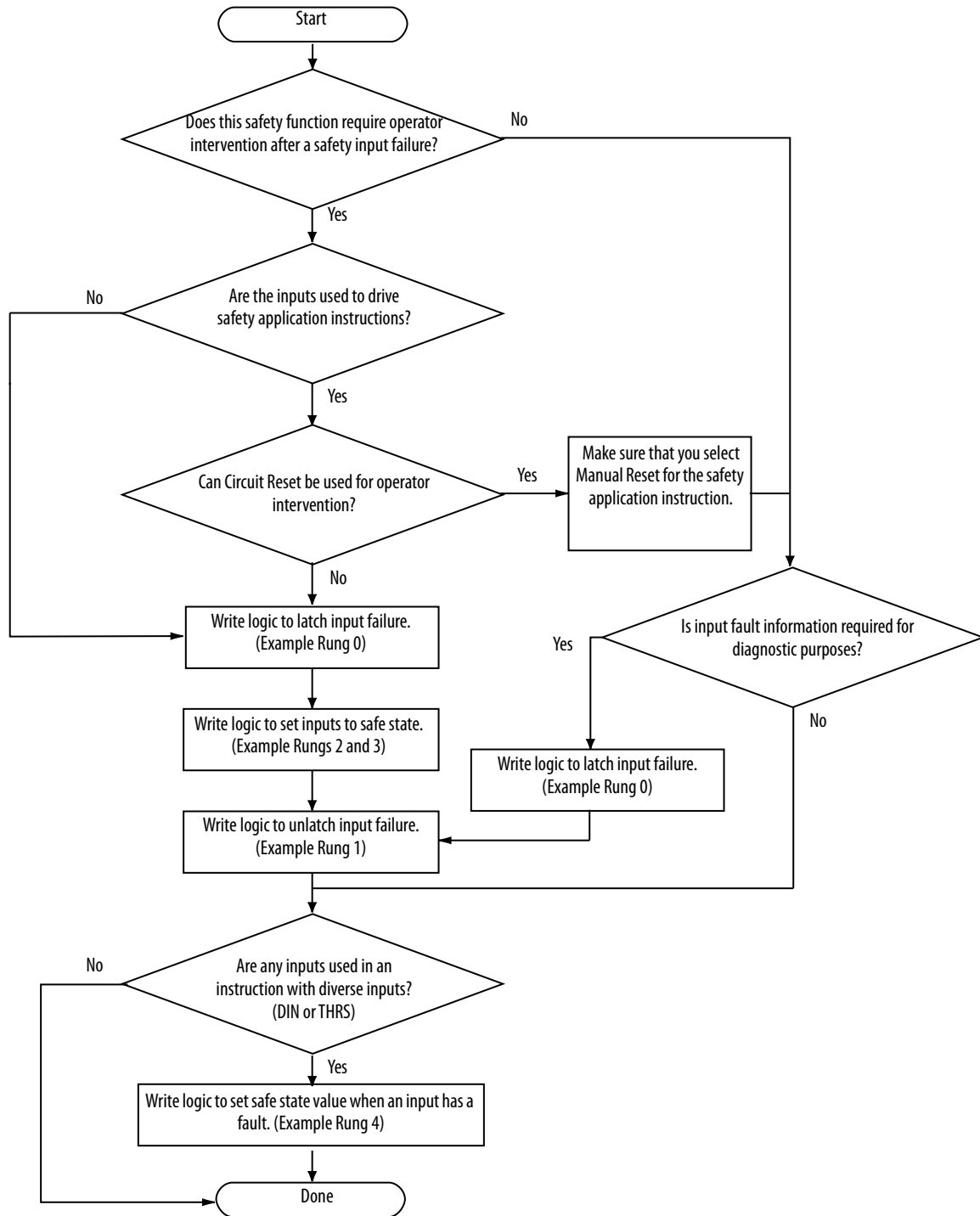
Figure 26 - Input Fault Latch and Reset Flowchart
