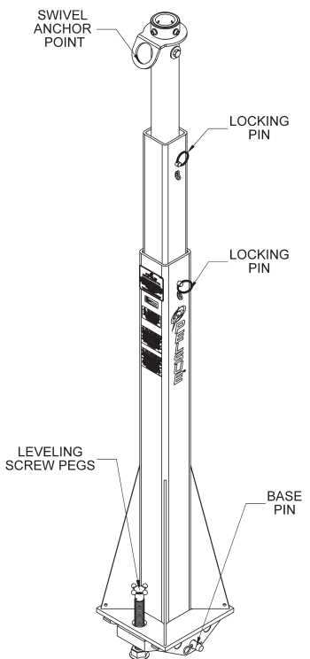
Figure #5.2a: #TFAT-11A Pre-Operation Inspection Points
