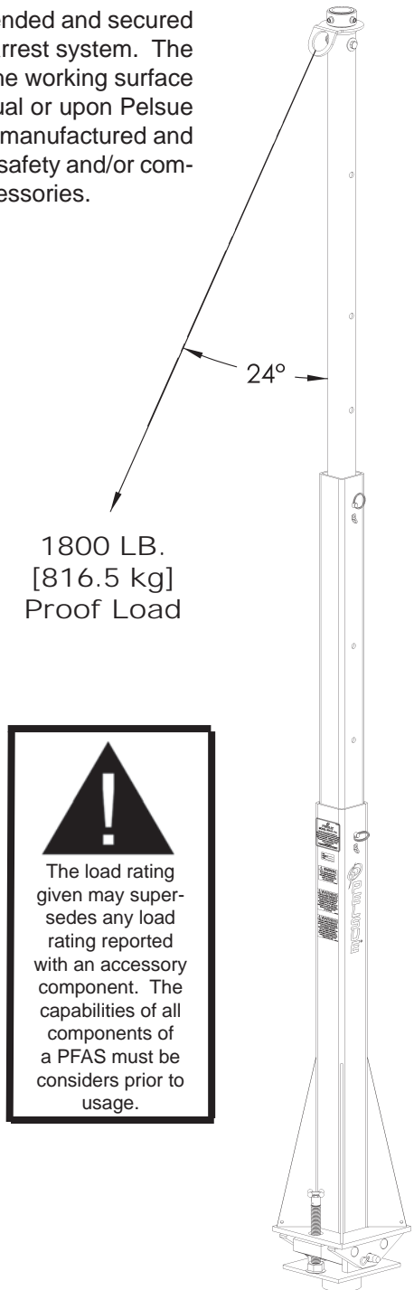
Figure #5.1a: Loading Diagram TFAT-11A
