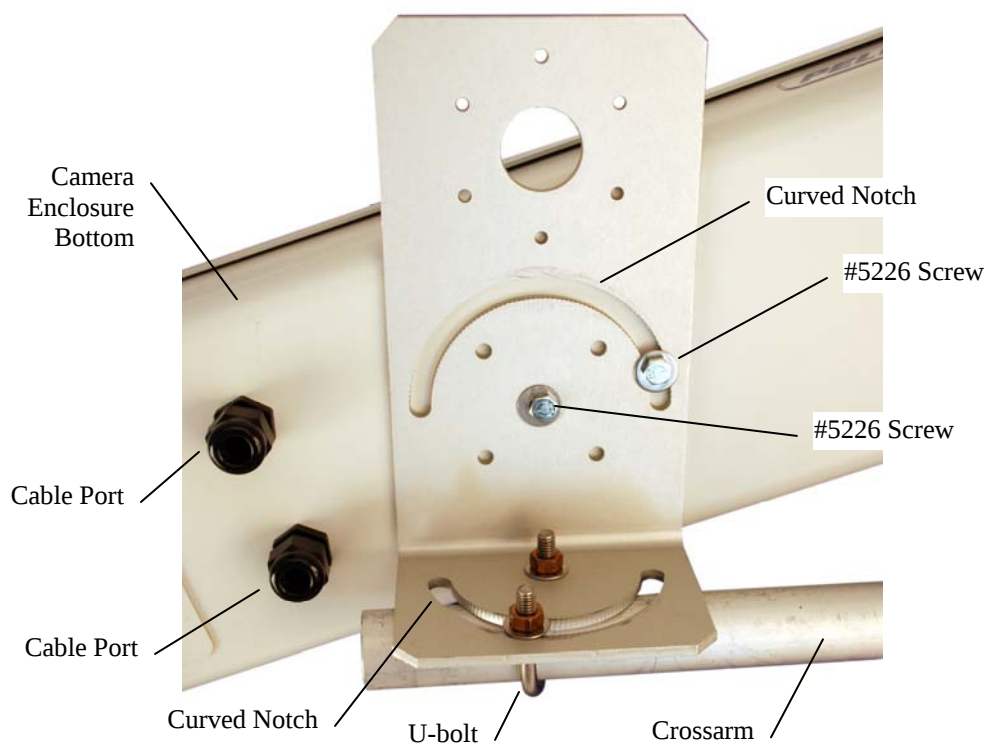
FIGURE 20. Camera Mount to Crossarm
