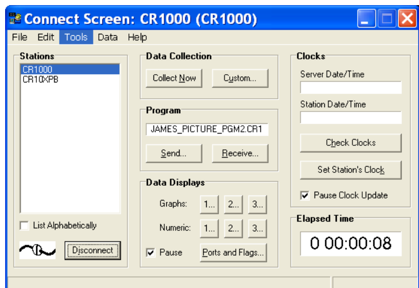
FIGURE 12. LoggerNet Screen
