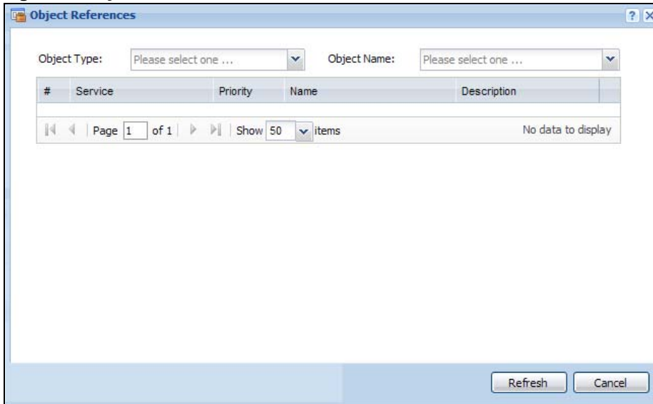
Figure 9 Object Reference
