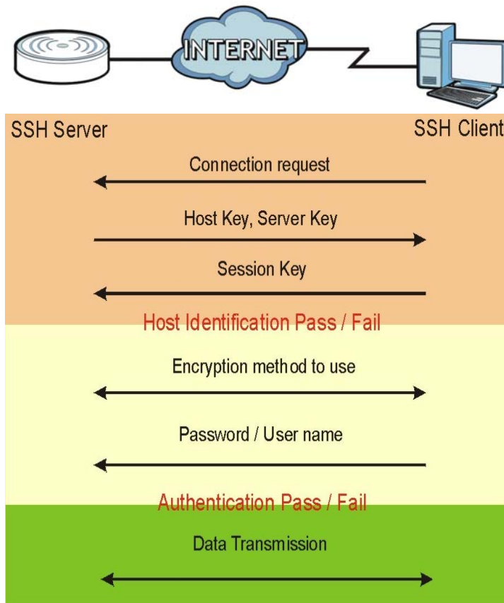
Figure 73 How SSH v1 Works Example
