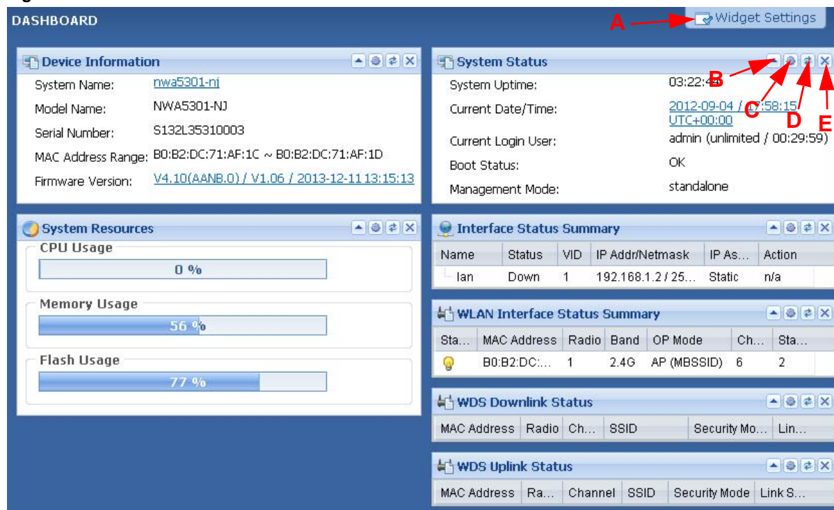
Figure 14 Dashboard
