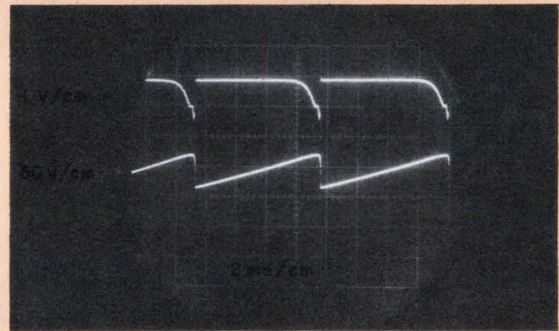
2. Positive-going blanking pulses (upper traces) have heights of about 80 V. The sweep voltage (lower traces) varies from 88 to 135 V. These photos are reversed from left to right.
