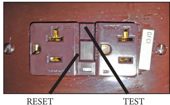
Figure 9-6: GFCI receptacle
