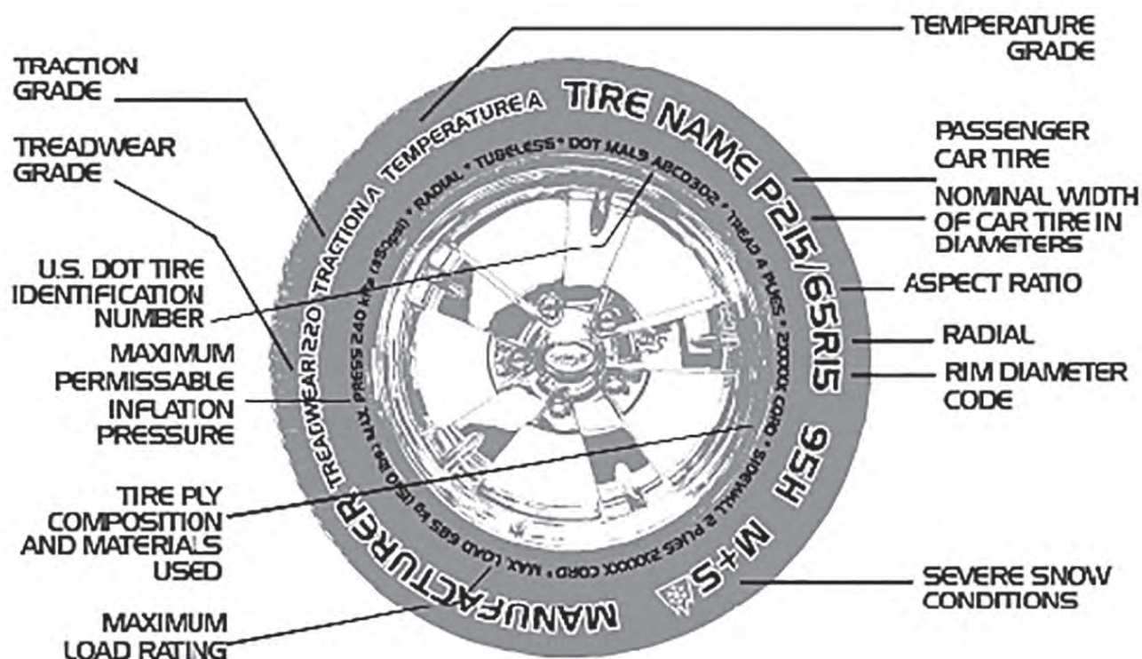
Figure 16-3: Tire information
