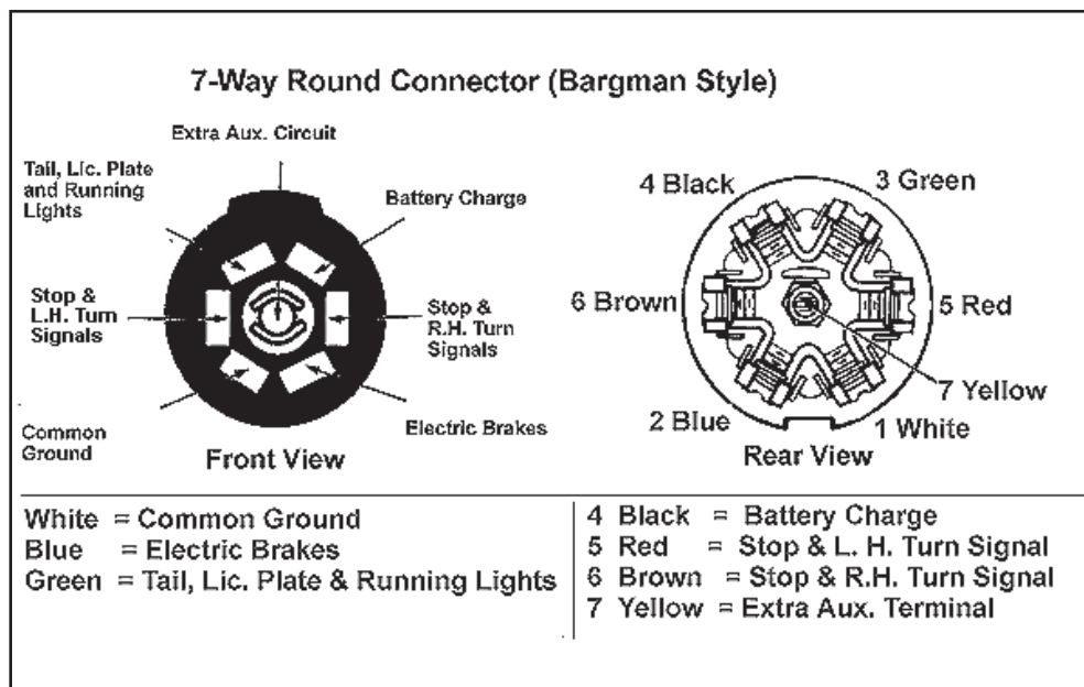
Figure 9-19: Seven-Pin towing connector
