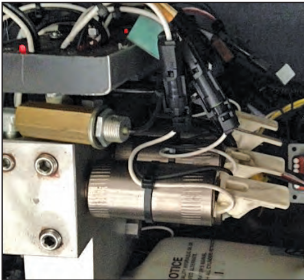
Figure 15-6: Closed valves
