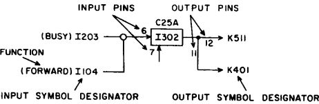
Figure 17. Input/Output Designations
