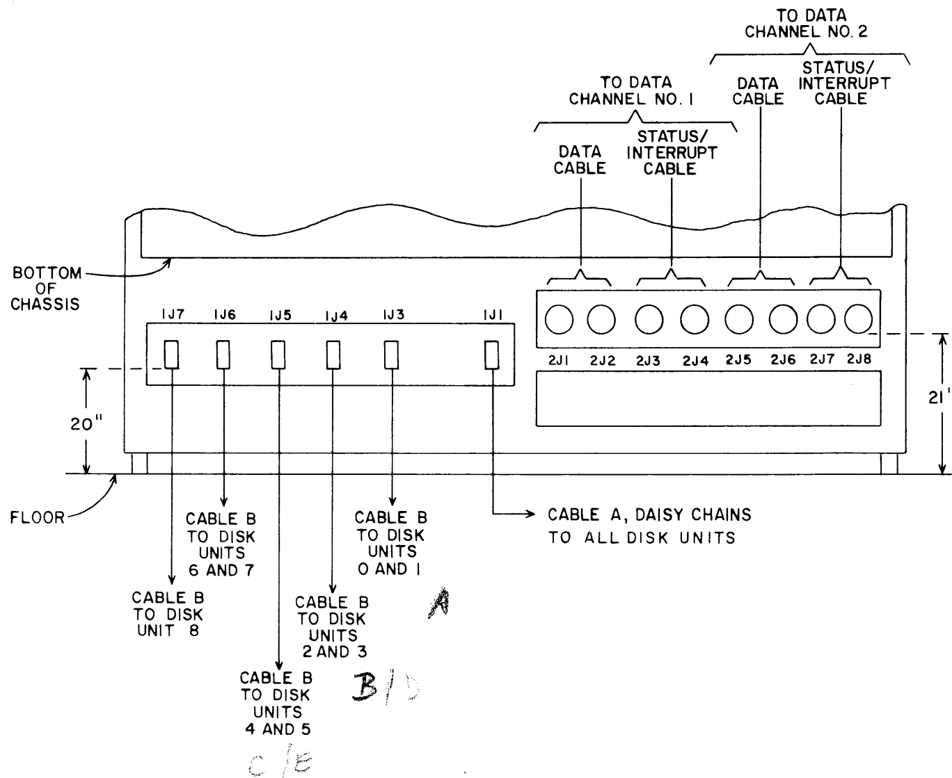
Figure 3-2. Connector Panel
