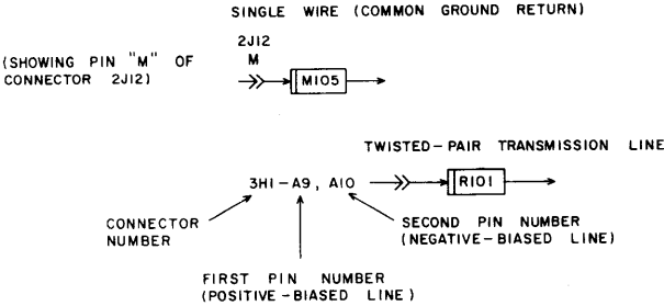
Figure 15. Cable Connections
