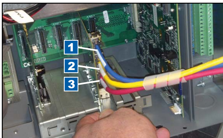
Figure 11. Install Ethernet Module In Slot 4
