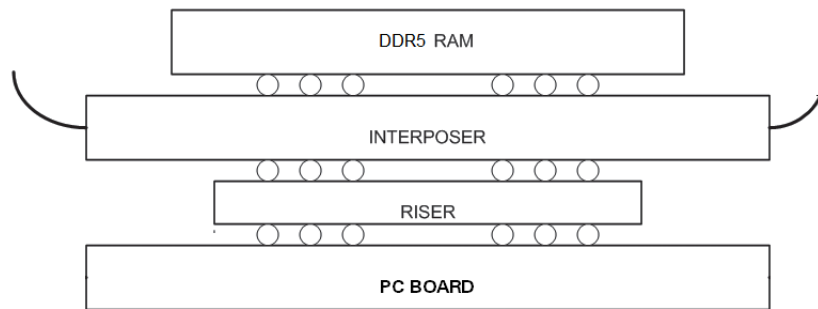
Figure 34 PC board, riser (or optional Grypper socket), interposer, and DRAM stack up
