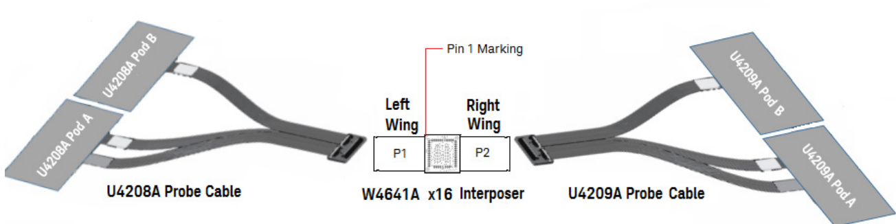
Figure 54 W4641A Interposer and U4208A / U4209A Probe Cable Connections
