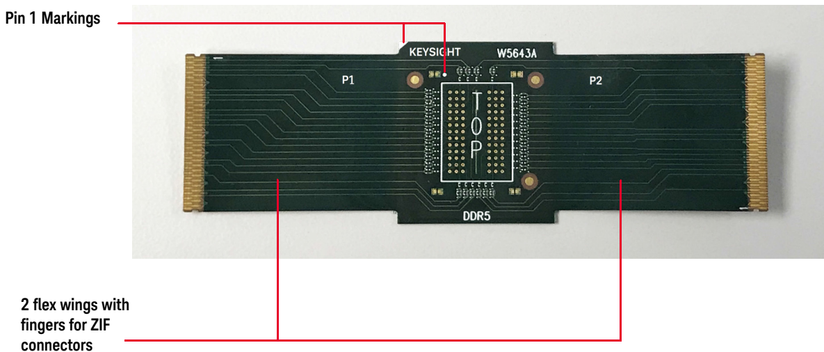
Figure 1 W5643A DDR5 x4/x8 BGA Interposer
