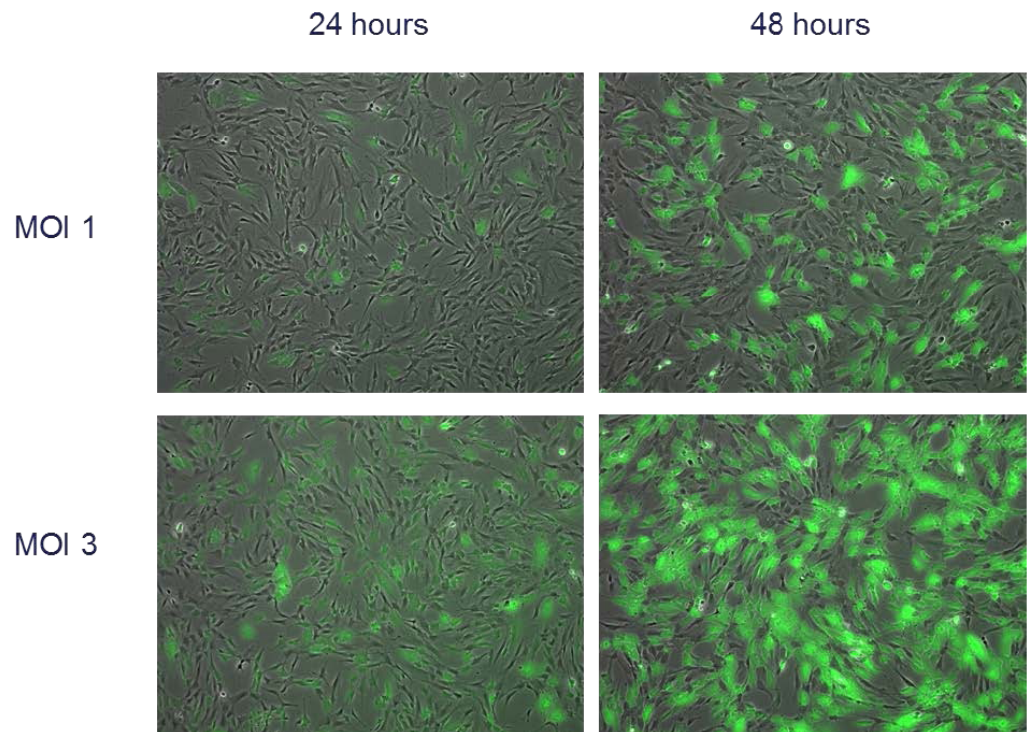
Figure 6 BJ HDFn cells transduced with the CytoTune™ -EmGFP Sendai Fluorescence Reporter at the indicated MOI (1 or 3) and at the indicated time post-transduction (24 or 48 hours).
