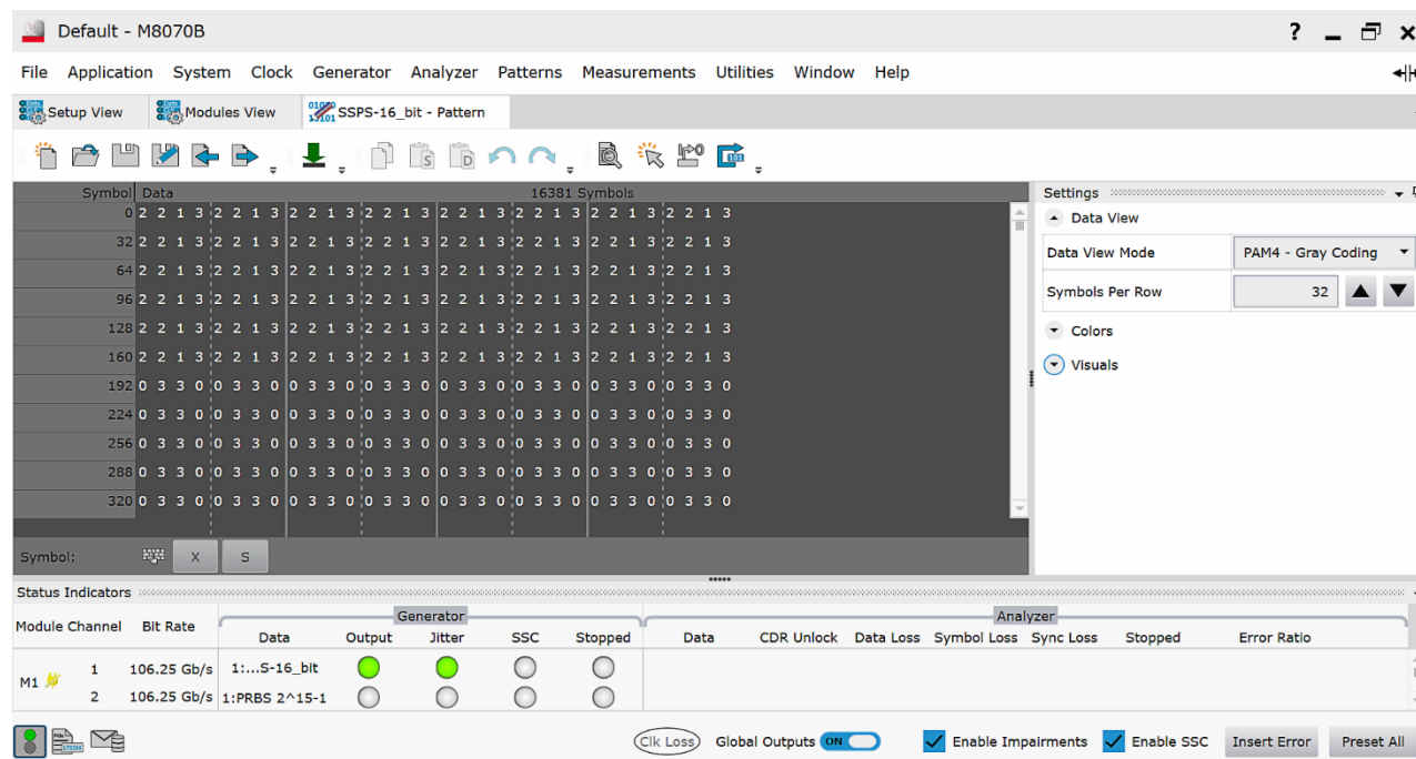
Figure 18. The pattern editor in the M8070B software allows editing NRZ bits and PAM4 symbols. The PAM4 symbol to bit mapping can be selected as Gray coded or custom with adjustable PAM4 levels. Quaternary PRBS, like QPRBS13-CEI or QPRBS31, according to CEI and IEEE standards can be selected as well as SSPRQ and PAM4 linearity test patterns.
