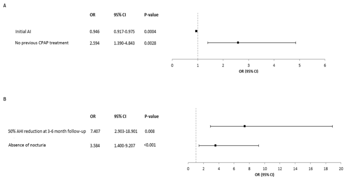
Fig. 5. Forest plot of multivariate analysis showing predictors of the apnoea-hypopnoea index (AHI) < 10/h (A) and continuation of treatment (B) after two years. AI, apnea index; CI, confidence interval; CPAP, continuous positive airway pressure; OR, odds ratio.
