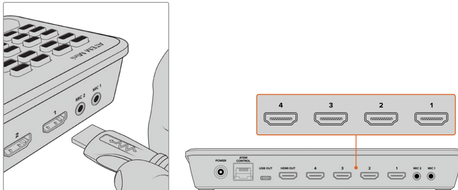
Plug HDMI sources into ATEM Mini's four HDMI inputs
