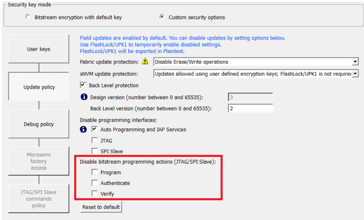
Figure 4-4. Locks to Protect Bitstream Programming Actions
