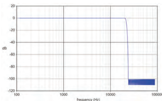
Fig 3. Frequency response of an example 4× interpolation filter
