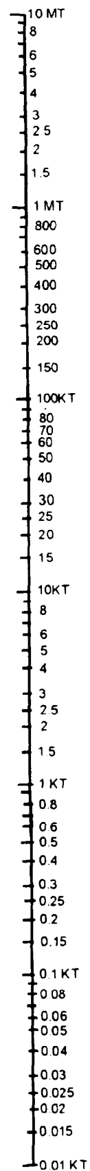
Figure 5-7.—Zone I downwind distance nomogram, used to calculate downwind distance from the effective downwind speed and weapon yield provided in an effective downwind forecast.
