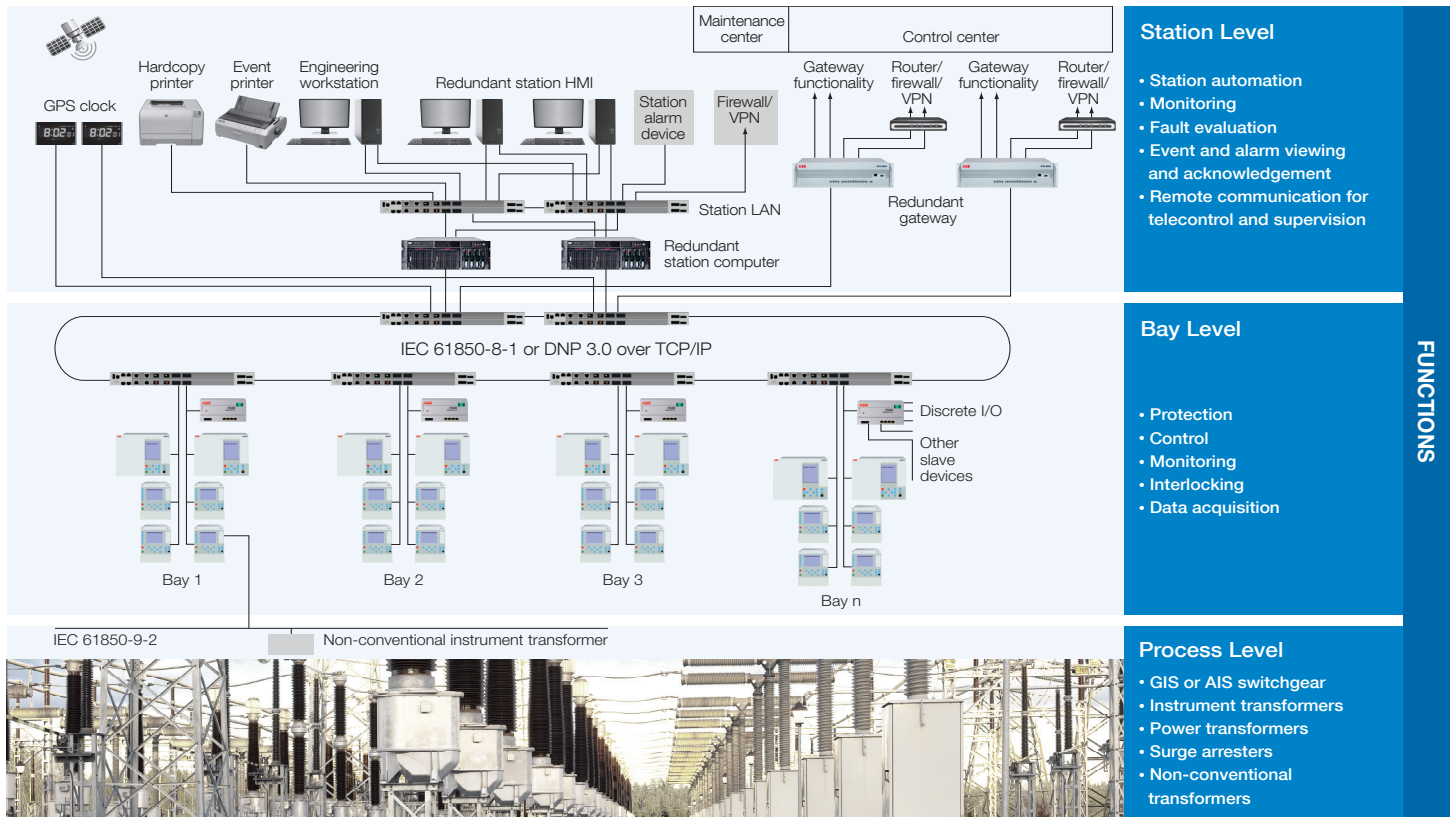
IEC 61850 architecture
