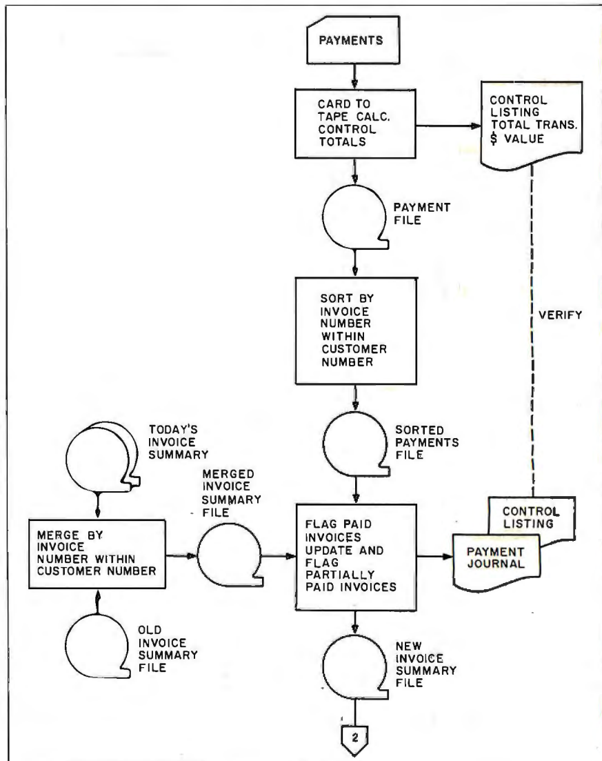
Figure 1: A systems flowchart—also a data-flow diagram.
