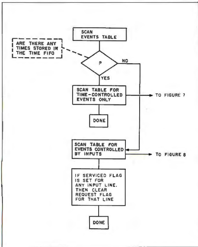
Figure 5: Execute Command flowchart.
