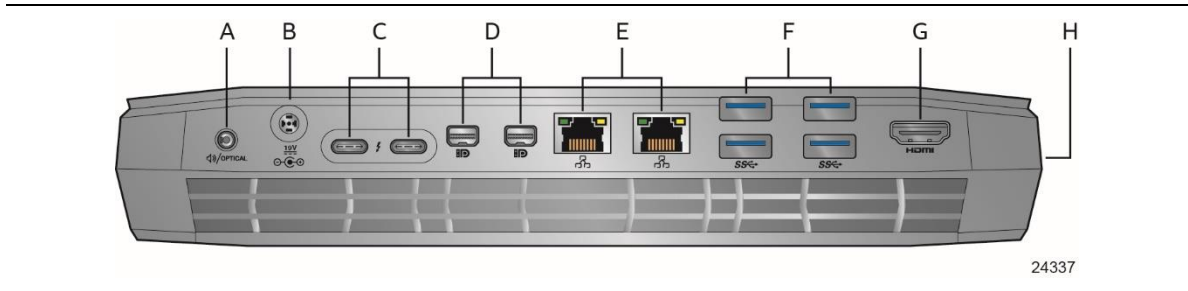
Figure 7. Back Panel Layout
