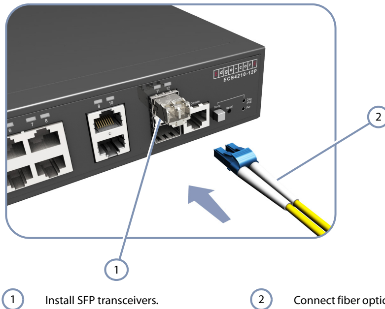
Figure 7: Making a Connection to an SFP Port
