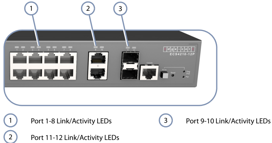
Figure 15: Port Status LEDs
