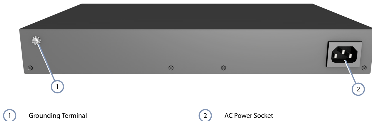
Figure 2: Rear Panel
