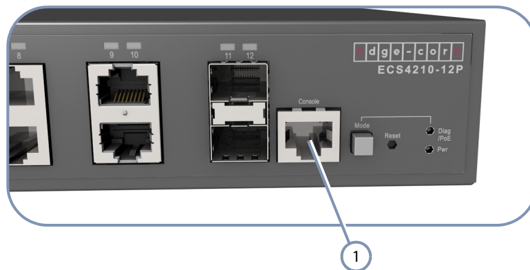
Figure 21: Console Port
