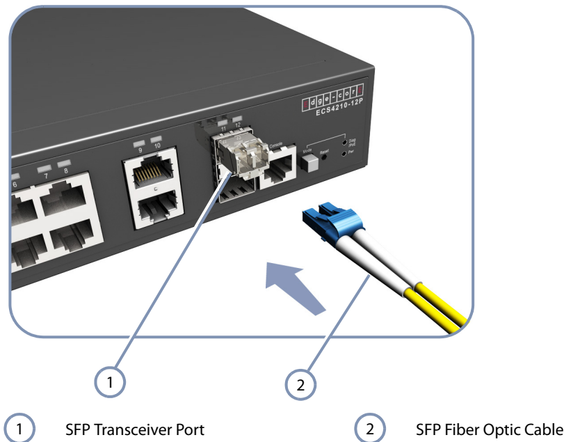
Figure 19: Making a Connection to an SFP Port
