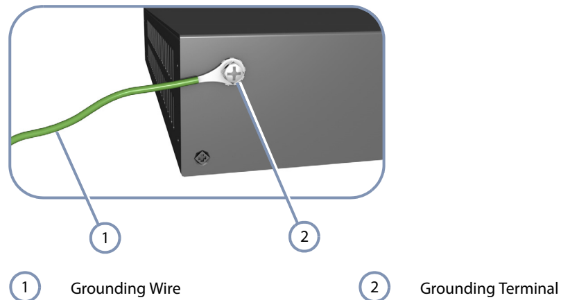
Figure 13: Grounding Terminal
