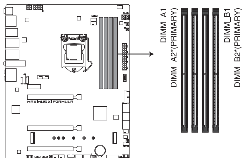
ROG MAXIMUS XI FORMULA 288-pin DDR4 DIMM socket
