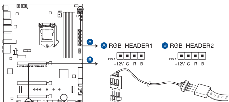
ROG MAXIMUS XI FORMULA RGB_HEADER connectors
