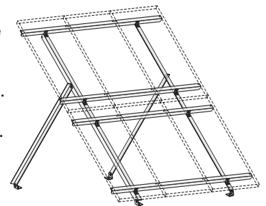
Roof/Ground Mount
