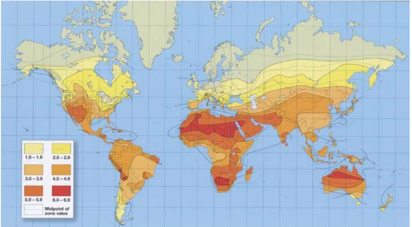
This map divides the world into six solar performance regions based on winter peak sun hours in the worst case month. A larger map in full color is located on the back cover of this catalog.
