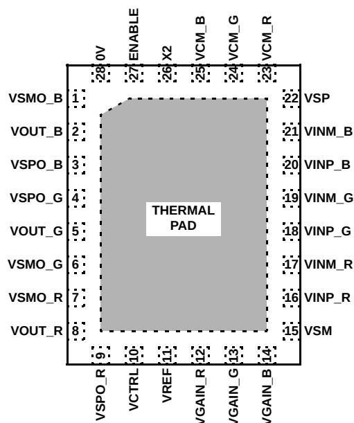
EL9112 (28 LD QFN) TOP VIEW
