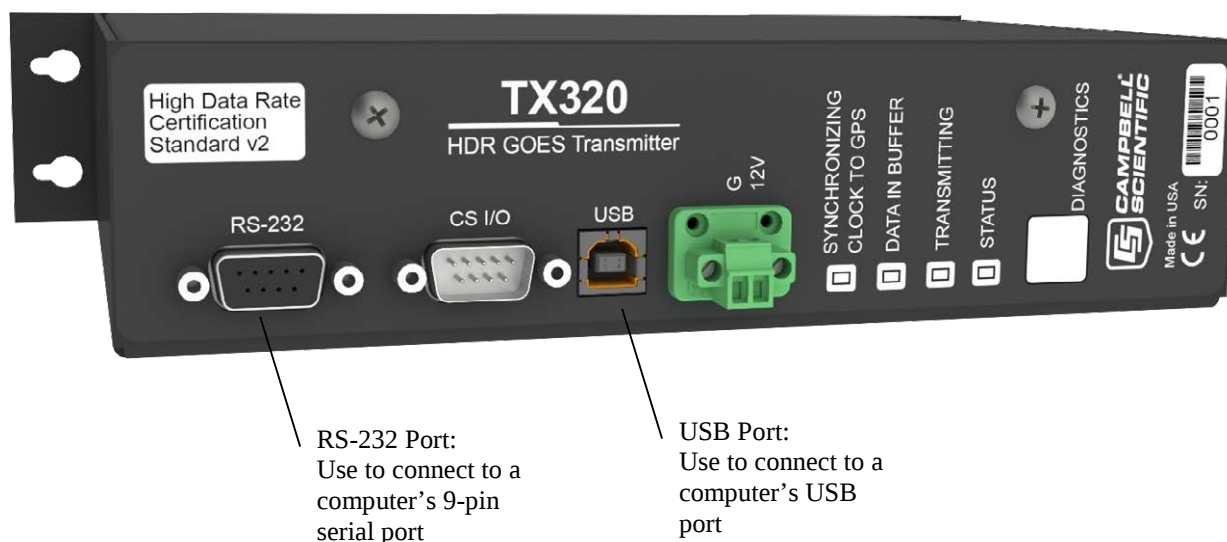
FIGURE 4-1. Ports used for computer connection
