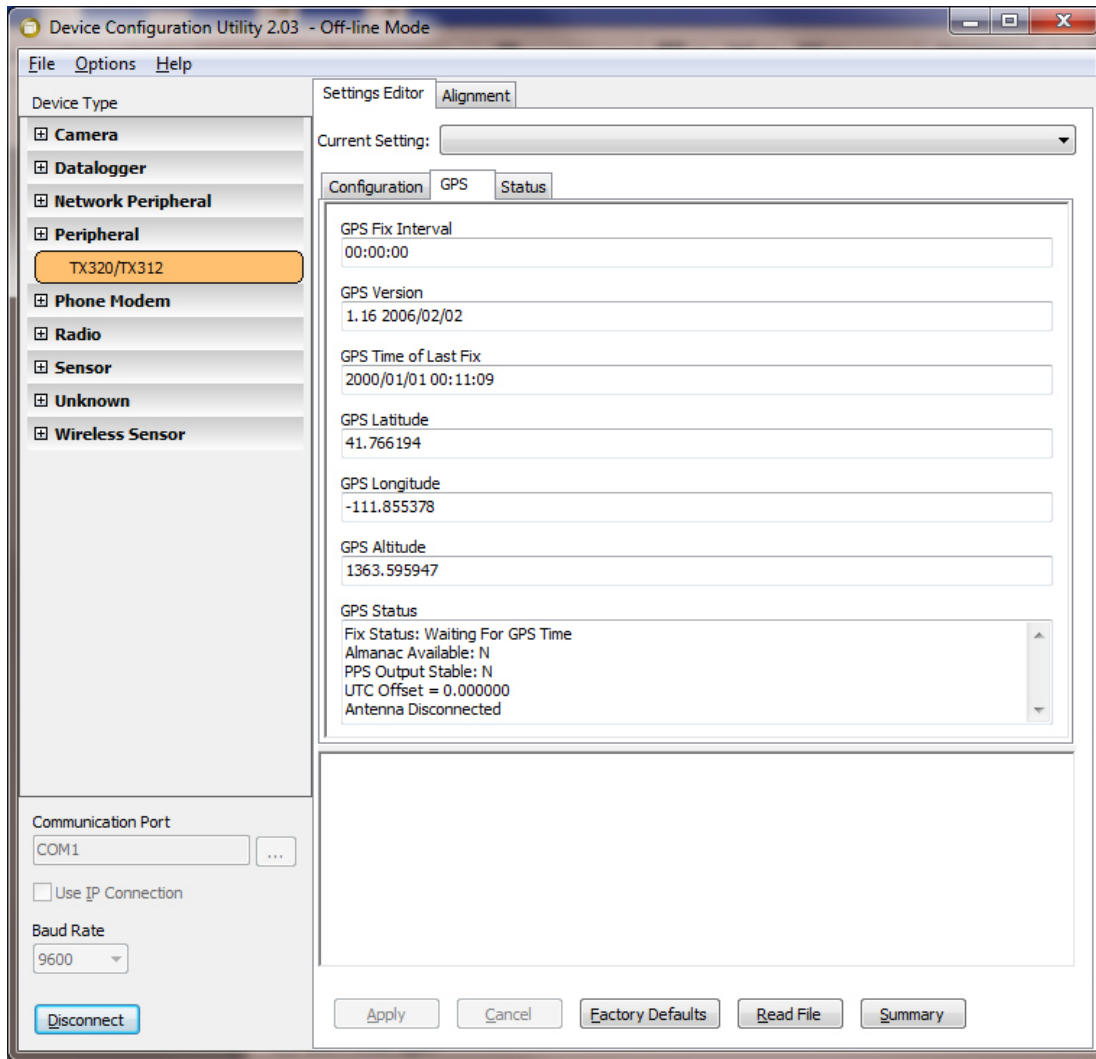
FIGURE 8-2. Settings Editor | GPS in Device Configuration Utility
