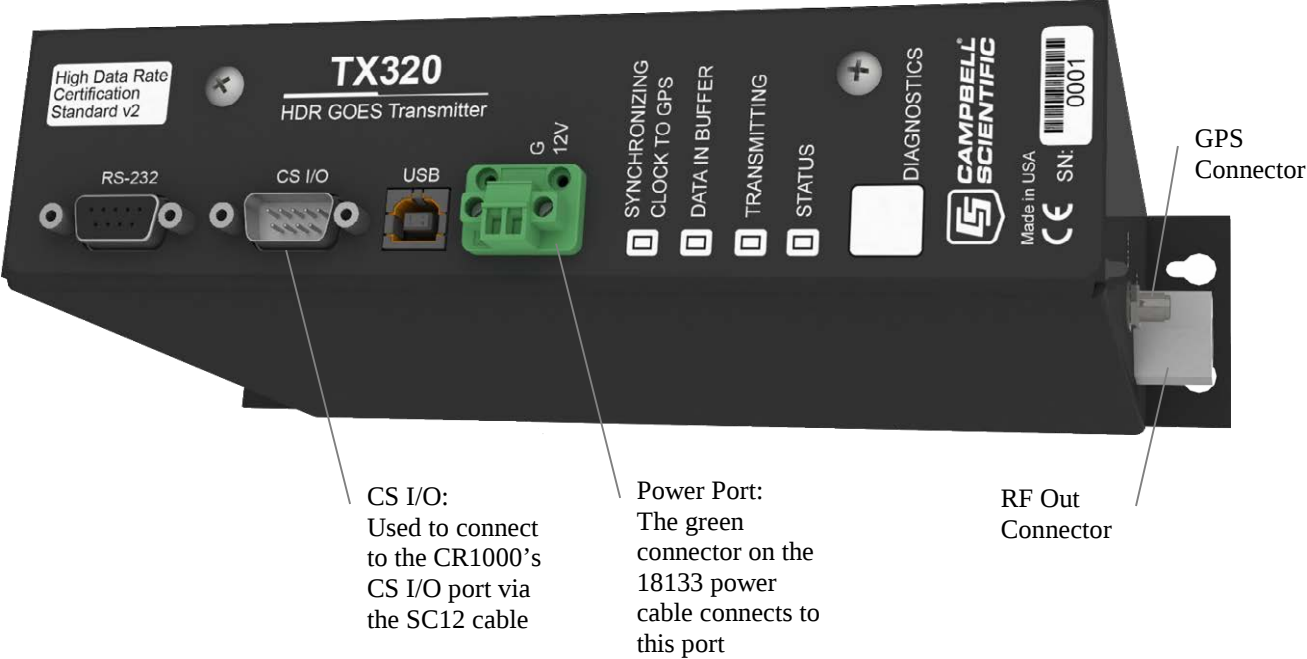
FIGURE 4-8. TX320 connectors
