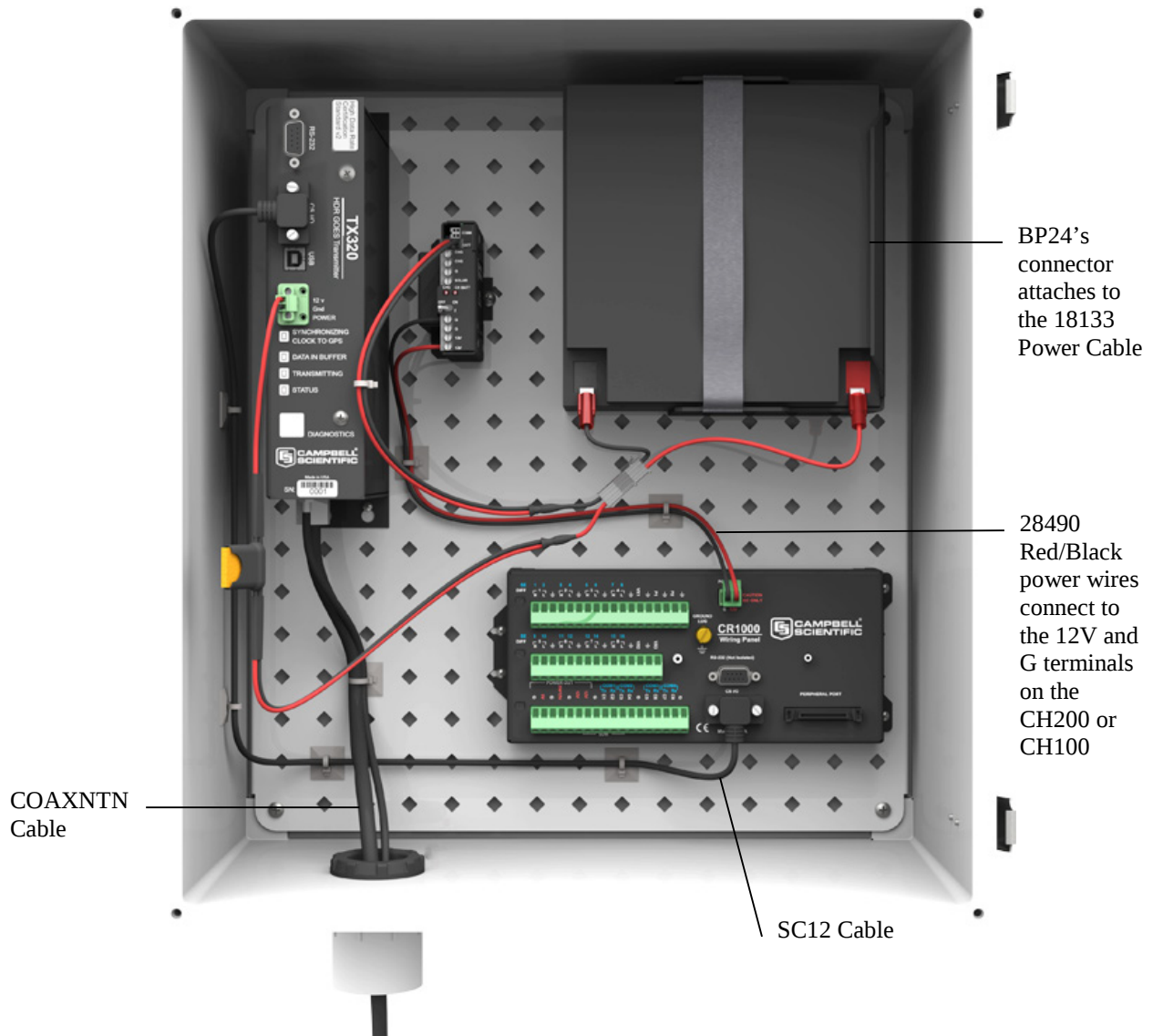
FIGURE 4-9. DCP enclosure
