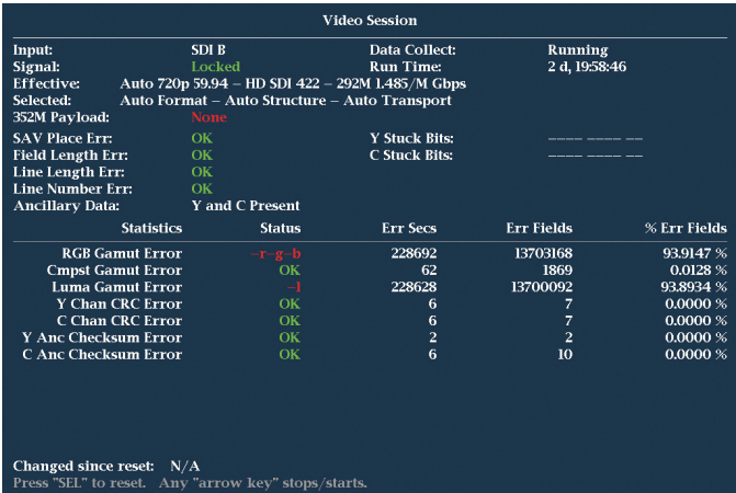
Figure 3. Status display showing CRC errors of an HD SDI signal.
