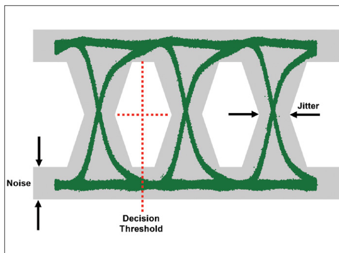
Figure 8. Eye decision threshold.
