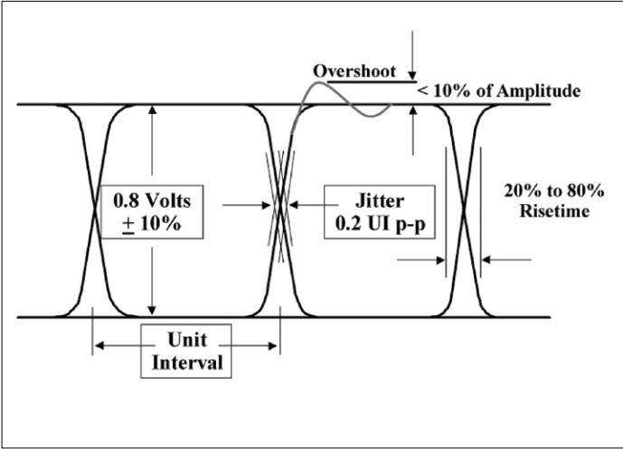
Figure 6. Eye measurement specifications.
