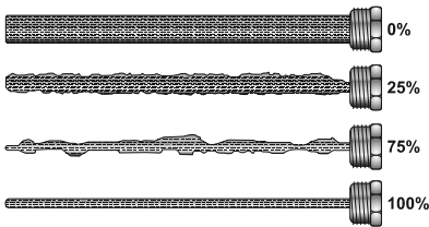
Fig. 8.5 Anode rod replacement chart
