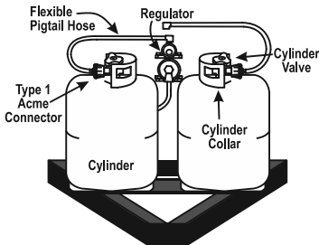
Fig. 7.6 Double cylinder
