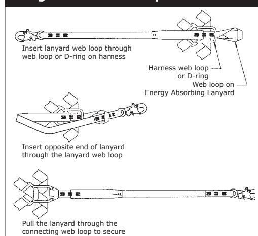
Figure 7 - Web Loop Connection
